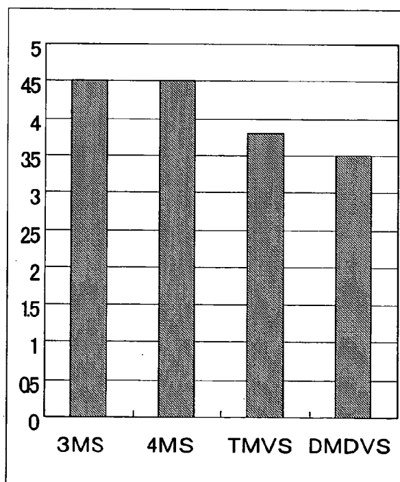
Fig.19 The dielectric constants of the SiCH films formed with various gases.
