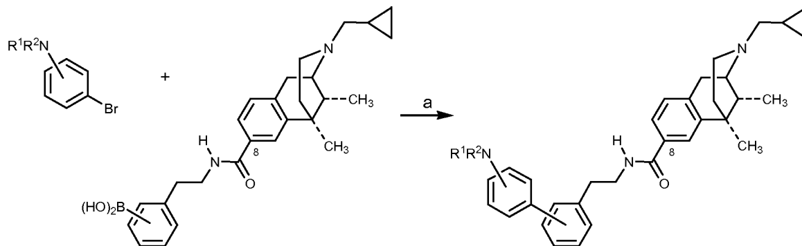
Scheme 3. Alternate method of syntheses of MV-E-126 related compounds via Suzuki coupling.
