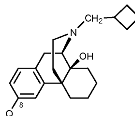
Butorphanol core
