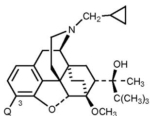
Buprenorphine core
