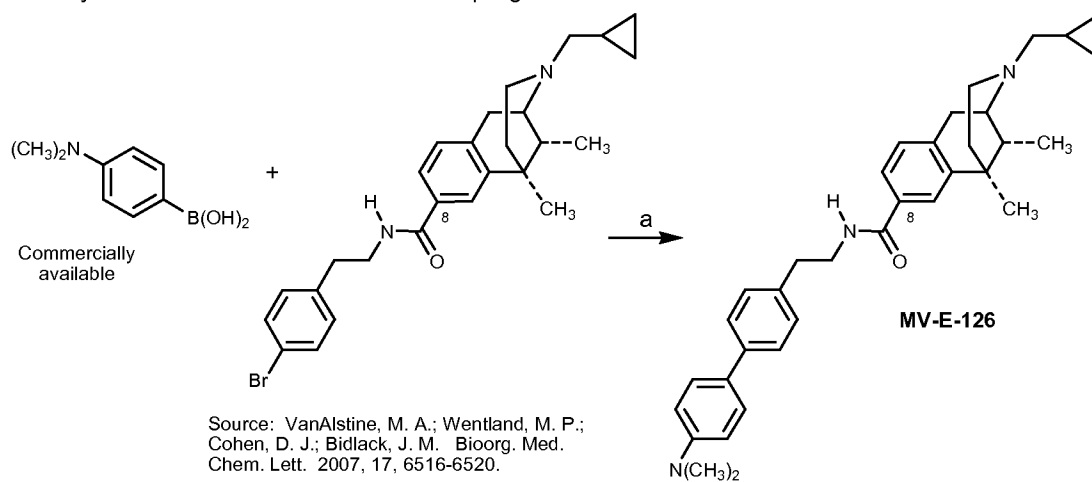
Scheme 1. Synthesis of MV-E-126 via Suzuki coupling.
