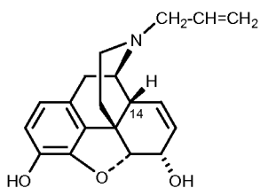
Nalorphine
