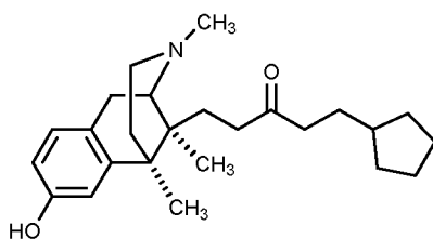
WIN 44,441
