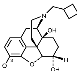
Nalbuphine core
