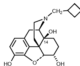
Nalbuphine
