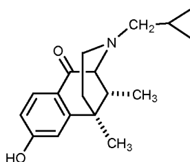
Ketocyclazocine
