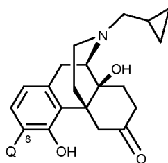
naltrexone ring opened
