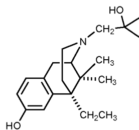
Bremazocine
