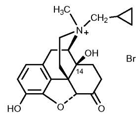
Methyl naltrexone
