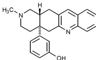
Registry number 173398-79-3
