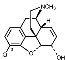
Morphine core
