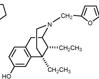
MR2266
