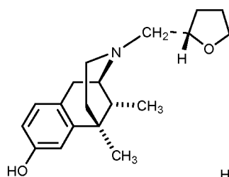
MR2034 - "Merz" core structure (opt. active)
