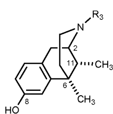
Cyclazocine, R_3 = \text{CH}_2\text{-C-C}_3\text{H}_5
