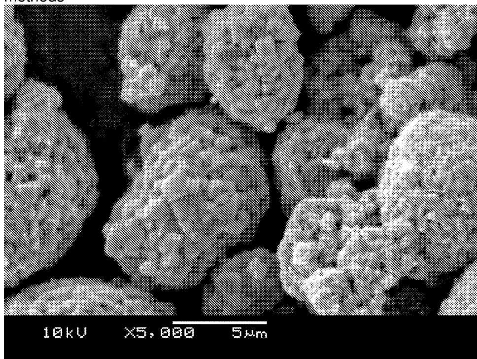
Fig. 7 (a) Aqueous solution coating of \text{Li}_3\text{AlO}_{2.1}\text{F}_{1.8} (Al:F:Al-O = 30:70 mol/mol) on NMC622 core particles
