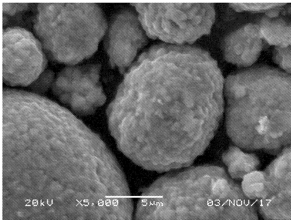
Fig. 7(e) Sol-gel coating of \text{Li}_{1.92}\text{Ti}_{0.47}\text{Al}_{0.16}\text{Zr}_{0.13}\text{Si}_{0.24}\text{O}_{2.49}\text{F}_{0.78} on NMC622 core particles
