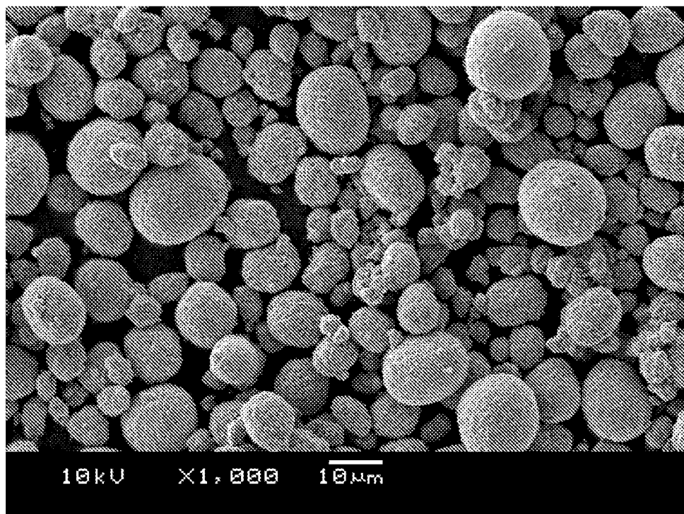
Fig. 3(c) NMC622 coated by \text{Li}_3\text{AlO}_{2.1}\text{F}_{1.8} (Al:F:Al-O = 30:70 mol/mol)
