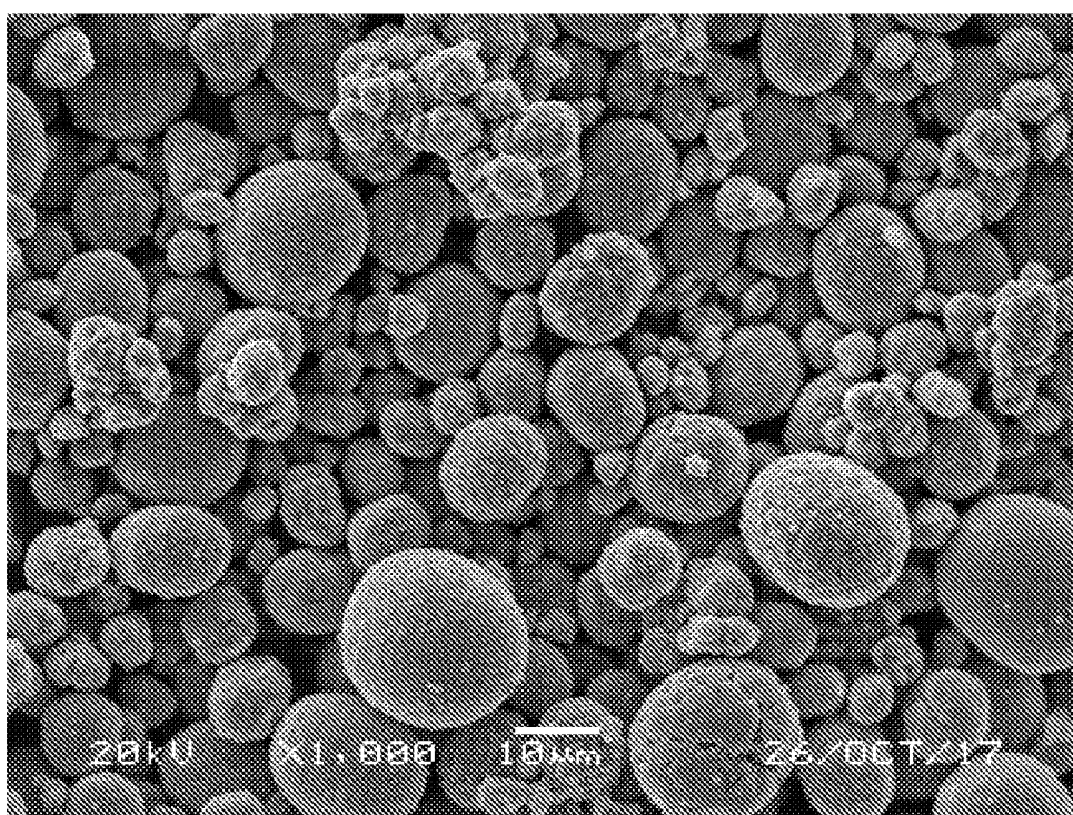
Fig. 7(d) Solid blending coating of \text{Li}_3\text{AlO}_{1.5}\text{F}_3 (Al-F:Al-O = 50:50 mol/mol) on NMC622 core particles
