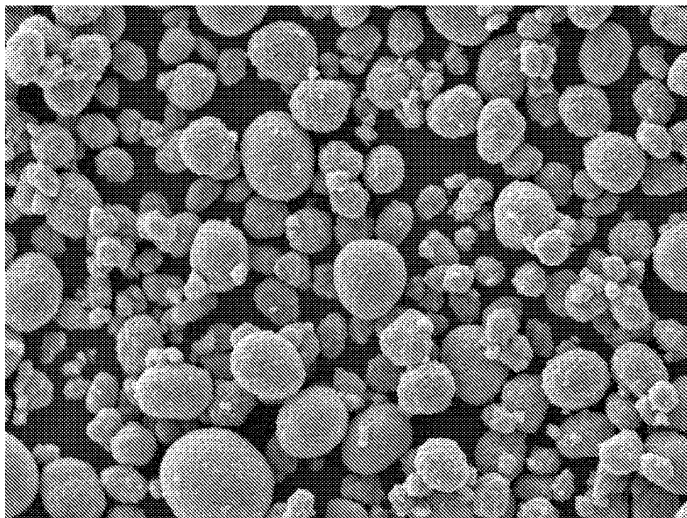
Fig. 3(a) NMC622 pristine
