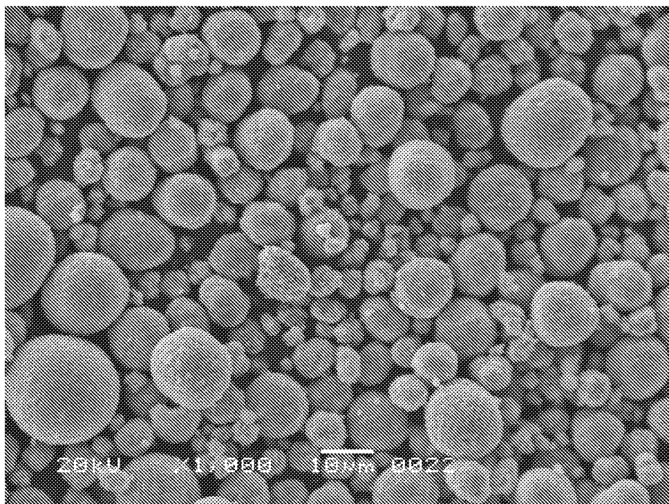
Fig. 3(e) NMC622 coated by \text{Li}_3\text{AlO}_{0.9}\text{F}_{4.2} (Al-F:Al-O = 70:30 mol/mol)
