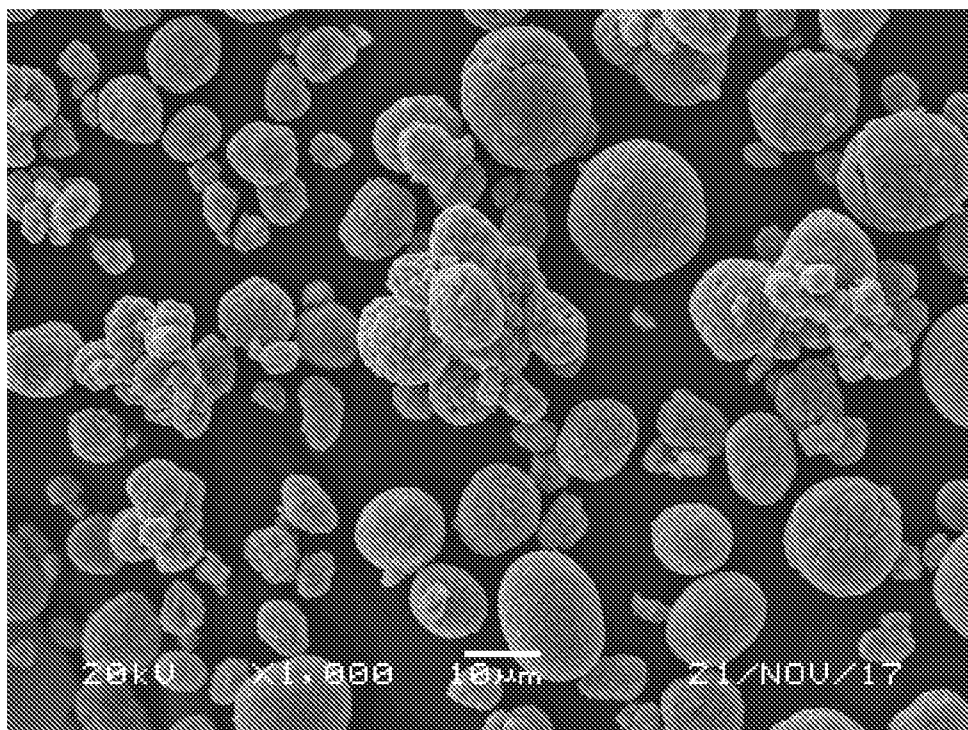
Fig. 3(b) NMC622 coated by \text{Li}_3\text{AlO}_{2.85}\text{F}_{0.3} (Al-F:Al-O = 5:95 mol/mol)
