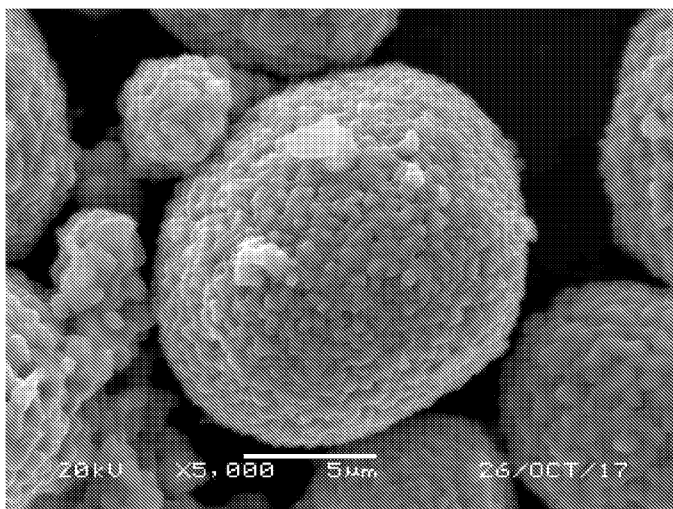
Fig. 7(b) Aqueous solution coating of \text{Li}_2\text{Ti}_{0.93}\text{Zr}_{0.07}\text{O}_{2.79}\text{F}_{0.42} on NMC622 core particles
