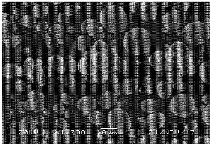
NMC622 coated by \text{Li}_3\text{AlO}_{2.85}\text{F}_{0.3} (Al-F:Al-O = 5:95 mol/mol)
