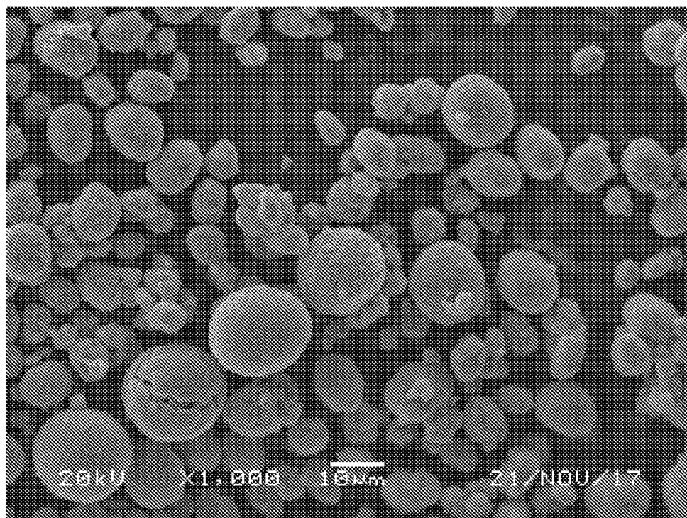
Fig. 3(d) NMC622 coated by \text{Li}_3\text{AlO}_{1.5}\text{F}_{3.0} (Al:F:Al-O = 50:50 mol/mol)
