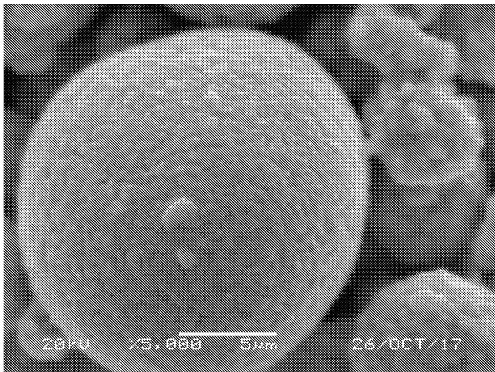
Fig. 7(c) Solvent solution coating of \text{Li}_3\text{AlO}_{0.9}\text{F}_{4.2} (Al-F:Al-O = 70:30 mol/mol) on NMC622 core particles
