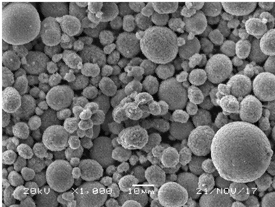
Fig. 3(g) NMC622 coated by \text{Li}_3\text{AlO}_{0.15}\text{F}_{5.7} (Al-F:Al-O = 95:5 mol/mol)
