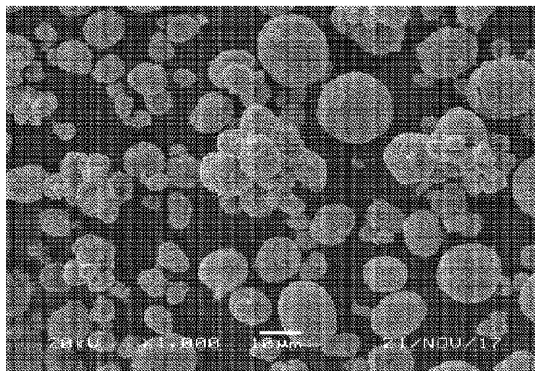
NMC622 coated by \text{Li}_3\text{AlO}_{2.85}\text{F}_{0.3} (Al:F:Al:O = 5:95 mol/mol)
