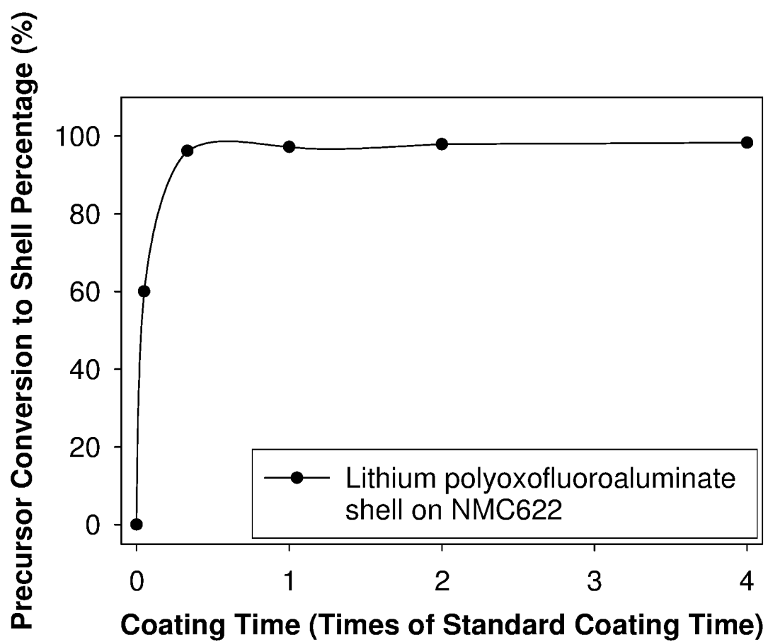
Fig.2 Precursor conversion percentage upon coating process time
