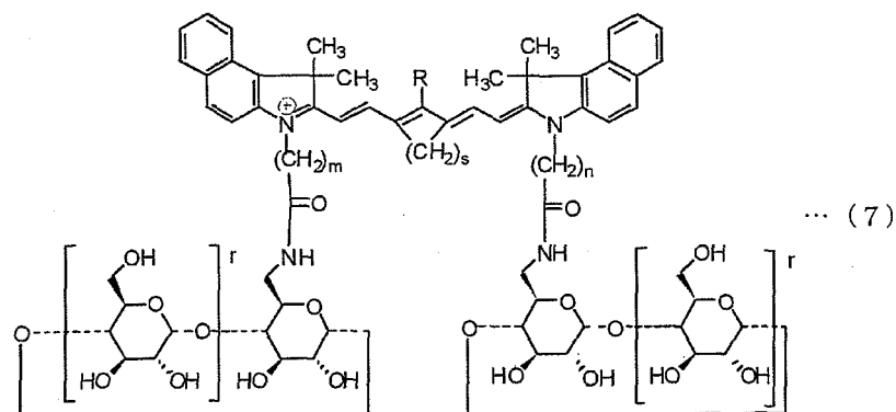
[Chem. 7]
