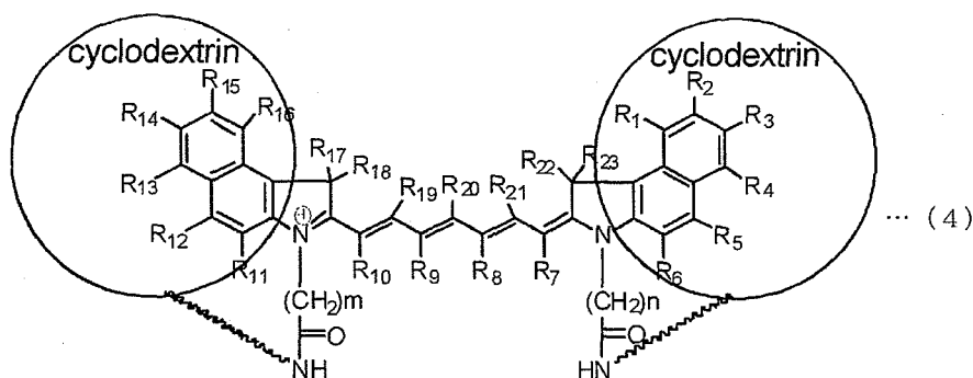
[Chem. 4]
