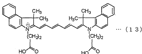
[Chem. 13]
