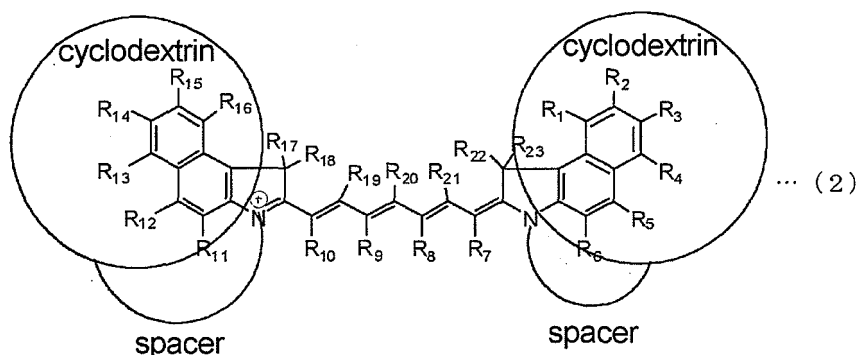
[Chem. 2]
