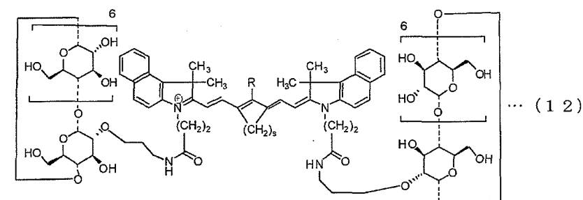
[Chem. 12]
