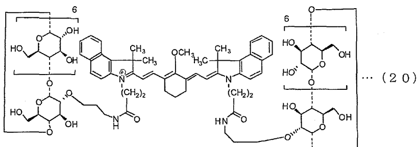
[Chem. 20]
