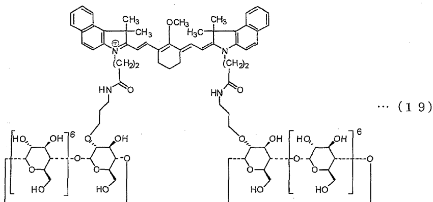
[Chem. 19]
