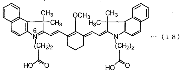
[Chem. 18]
