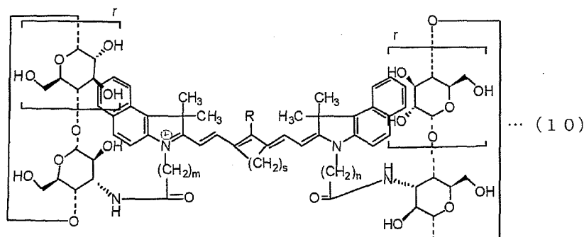
[Chem. 10]
