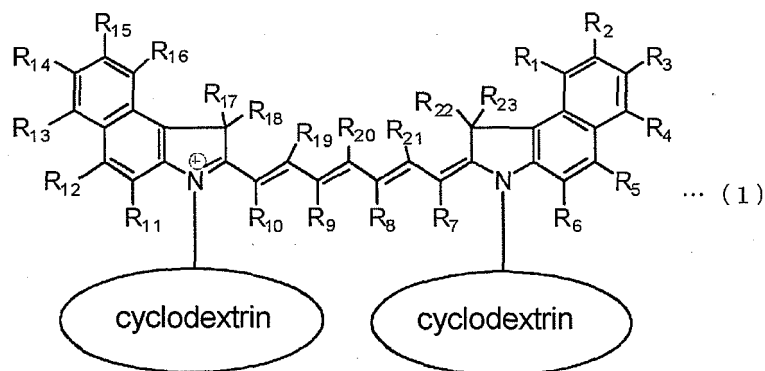
[Chem. 1]
