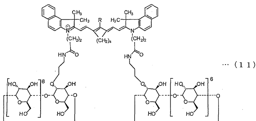
[Chem. 11]
