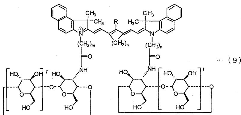
[Chem. 9]
