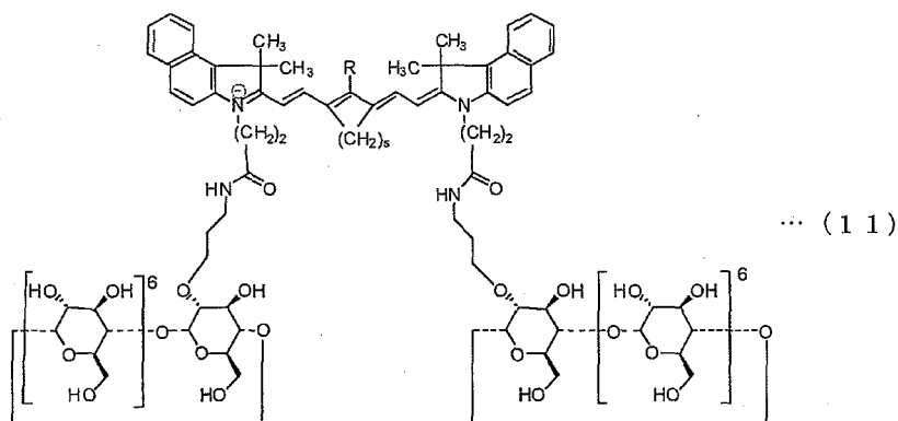
[Chem. 11]
