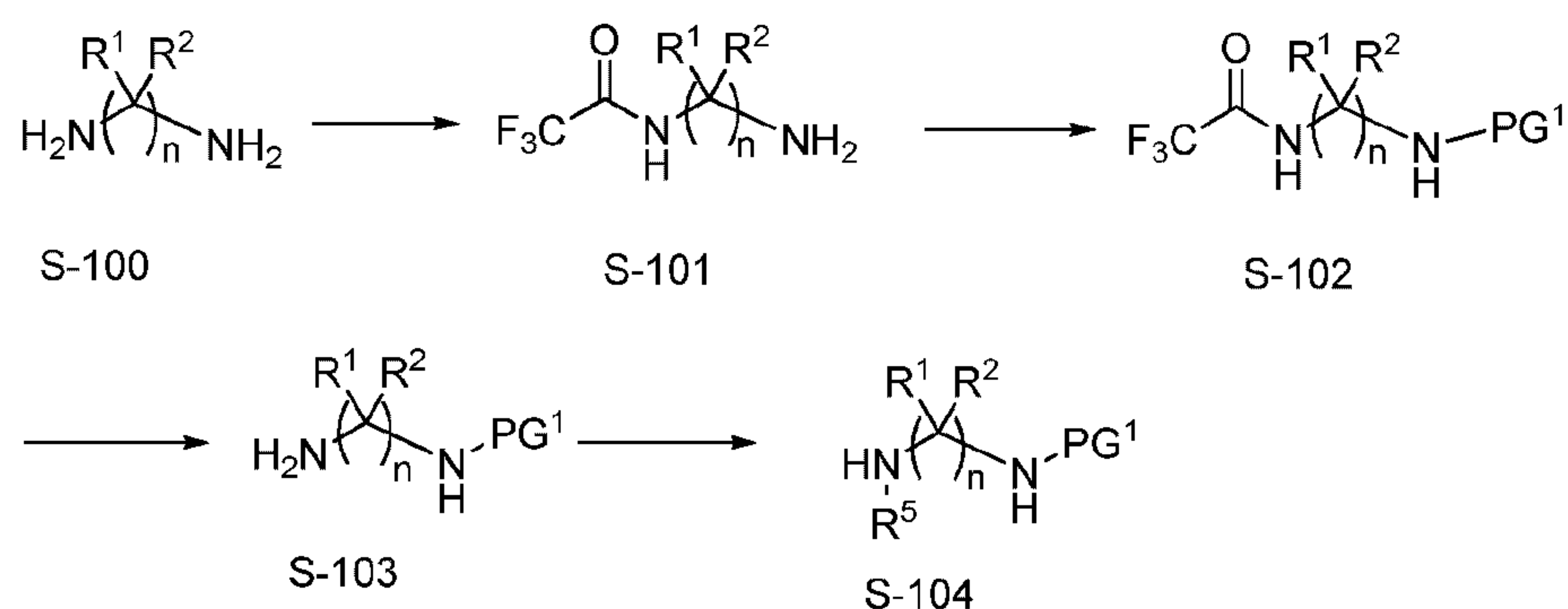
Scheme 1
