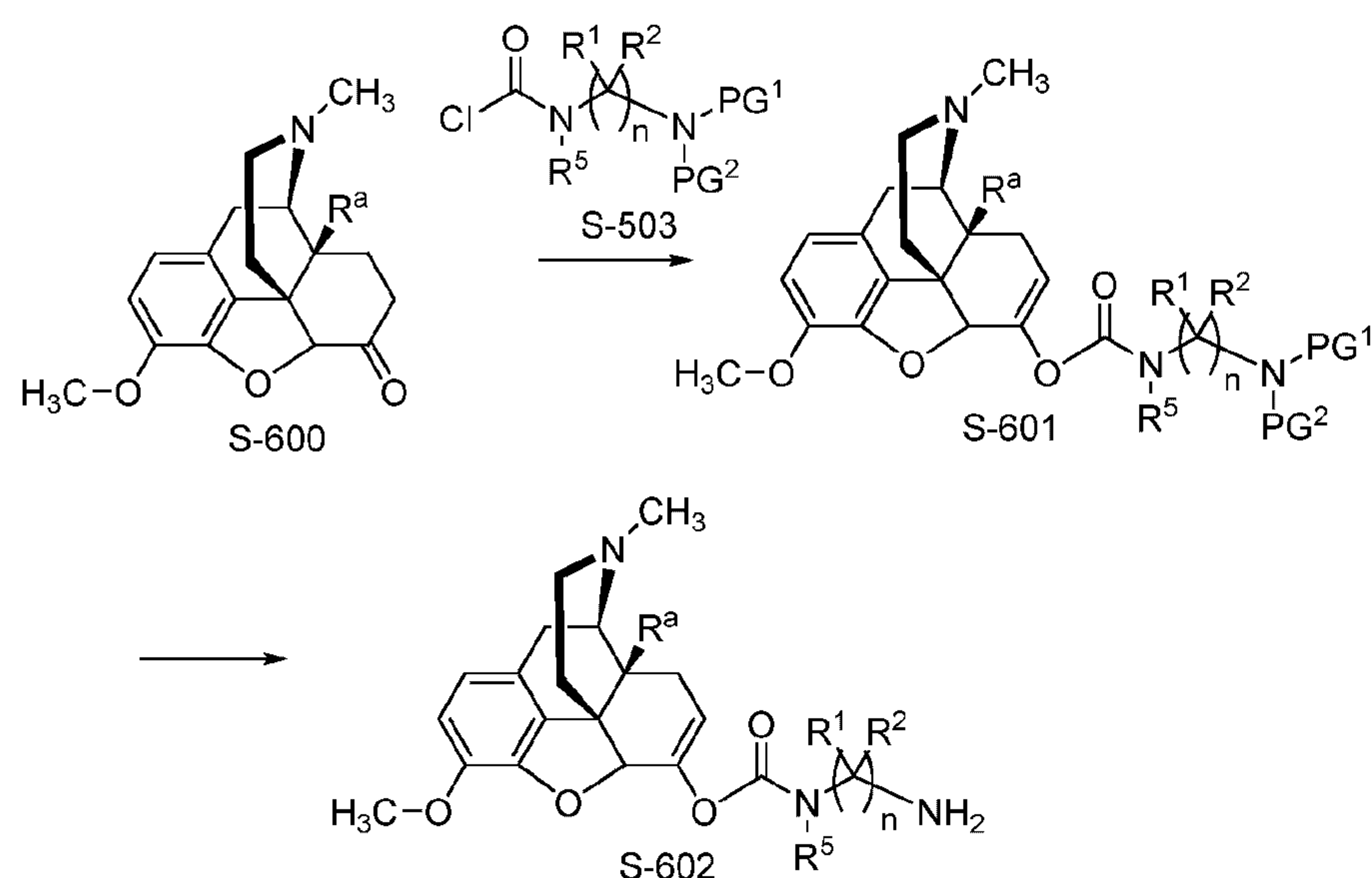
Scheme 6
