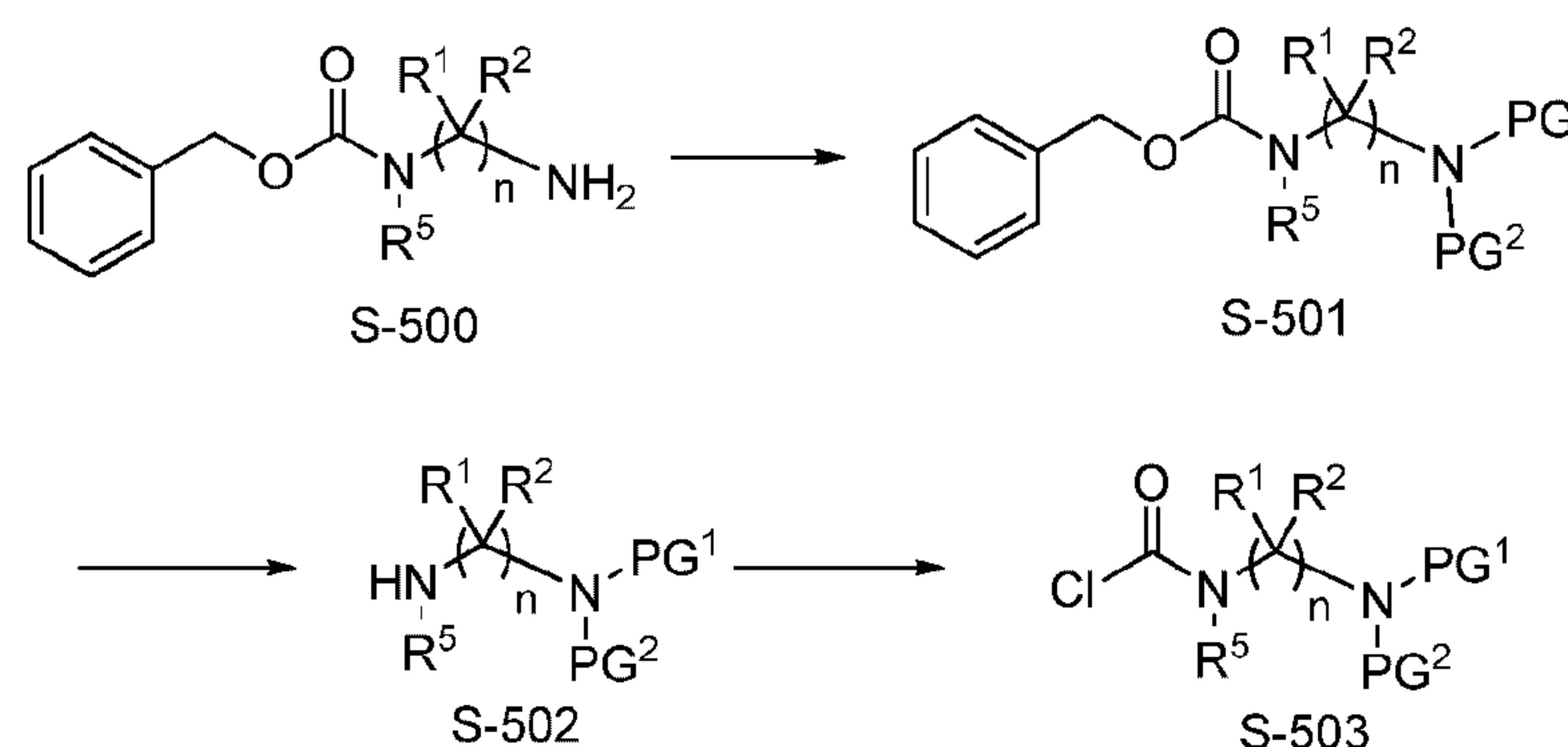
Scheme 5
