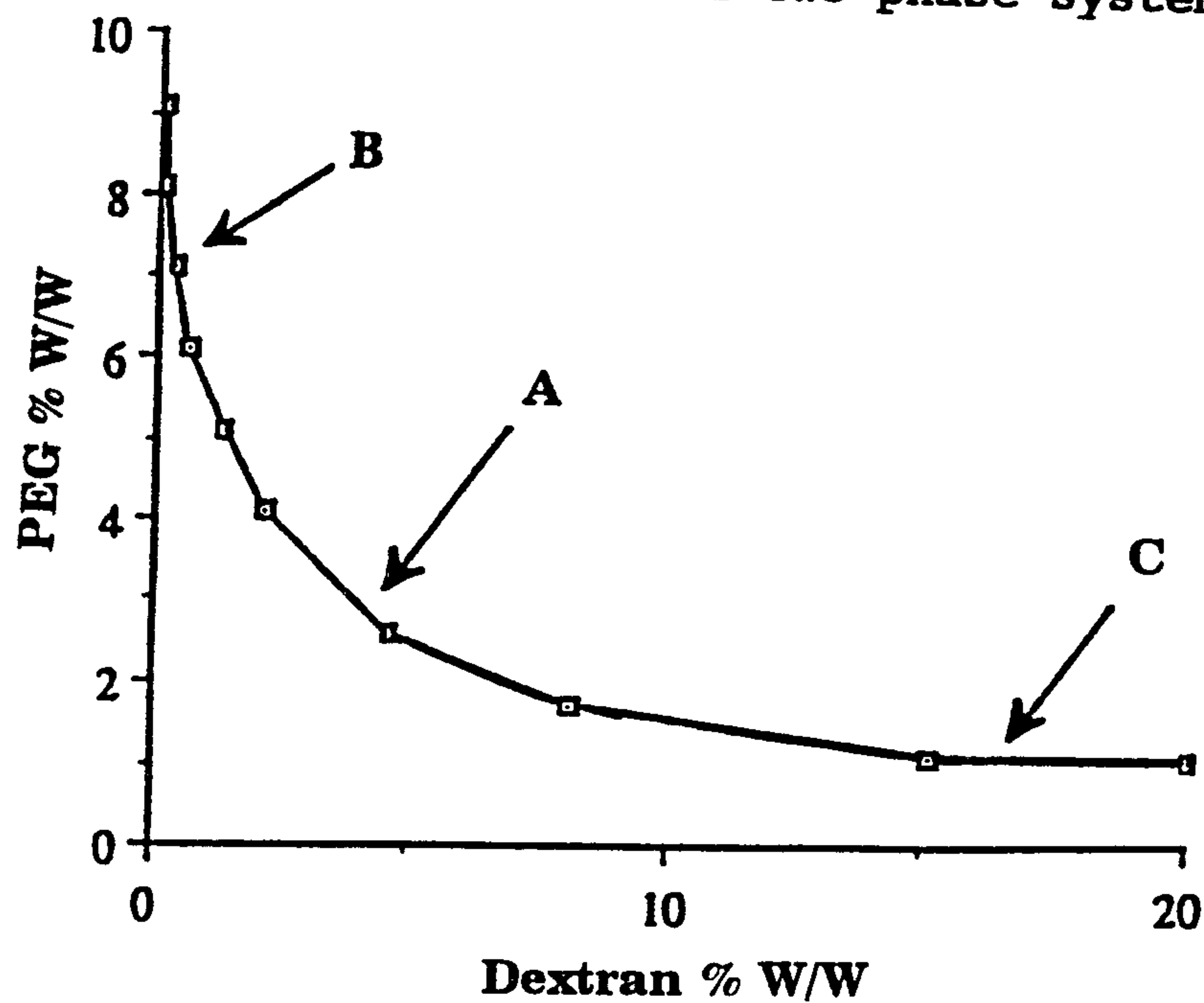
FIG. 1 Examples of a phase diagram of traditional two-phase systems.
