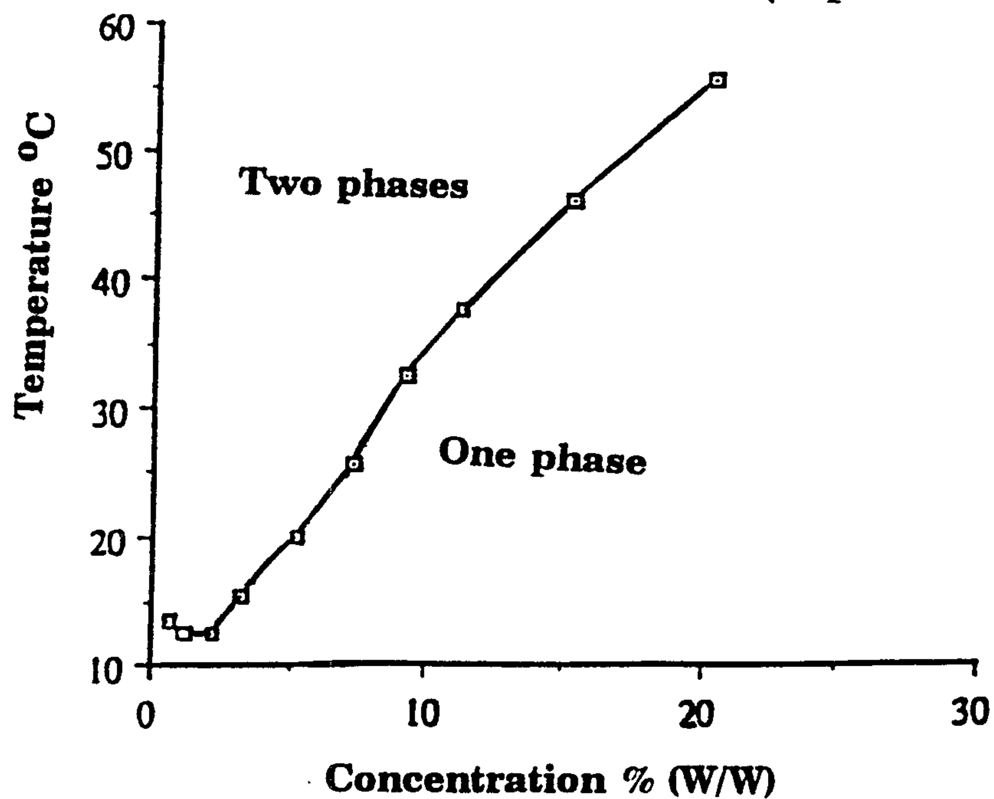
FIG. 2 Phase diagram for a temperature-induced phase separation (Dapral 210).
