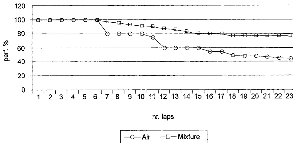
Tyre performance
