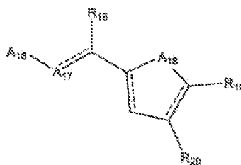
Formula V
