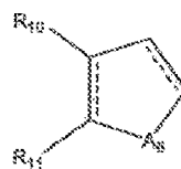
Formula III
