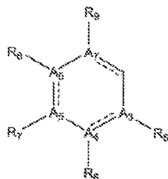
Formula II
