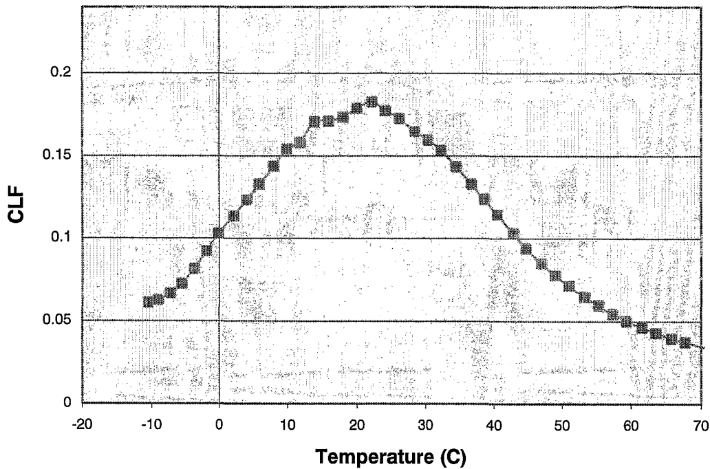
Figure 1. Oberst test result of example 1
