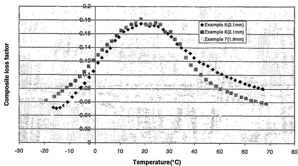
Figure 4. Oberst Test Results of Examples 5, 6 and 7
