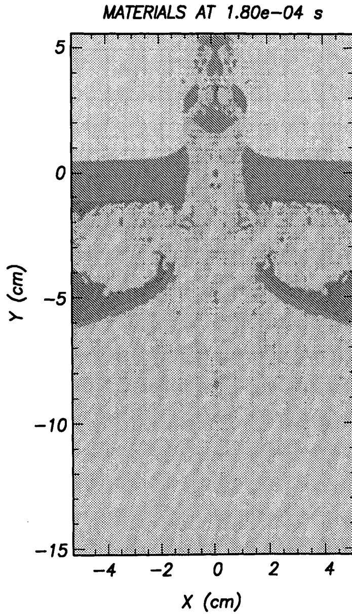
CTH SIMULATION WITH COPPER INSERT SHOWS A 15% LARGER HOLE SIZE IN CASING
