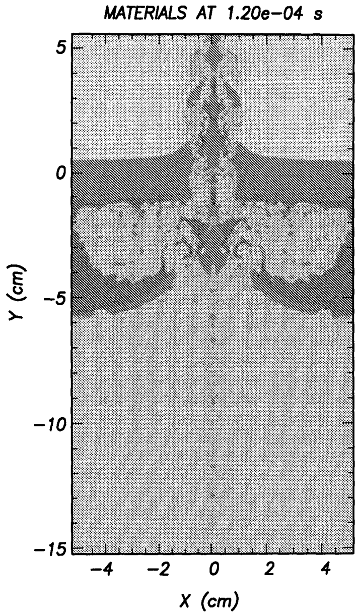
CTH SIMULATION FOR CONVENTIONAL LINER WITH NO INSERT
