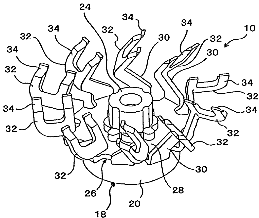
FIG. 10 PRIOR ART
