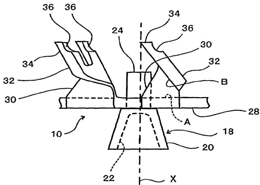
FIG. 12 PRIOR ART
