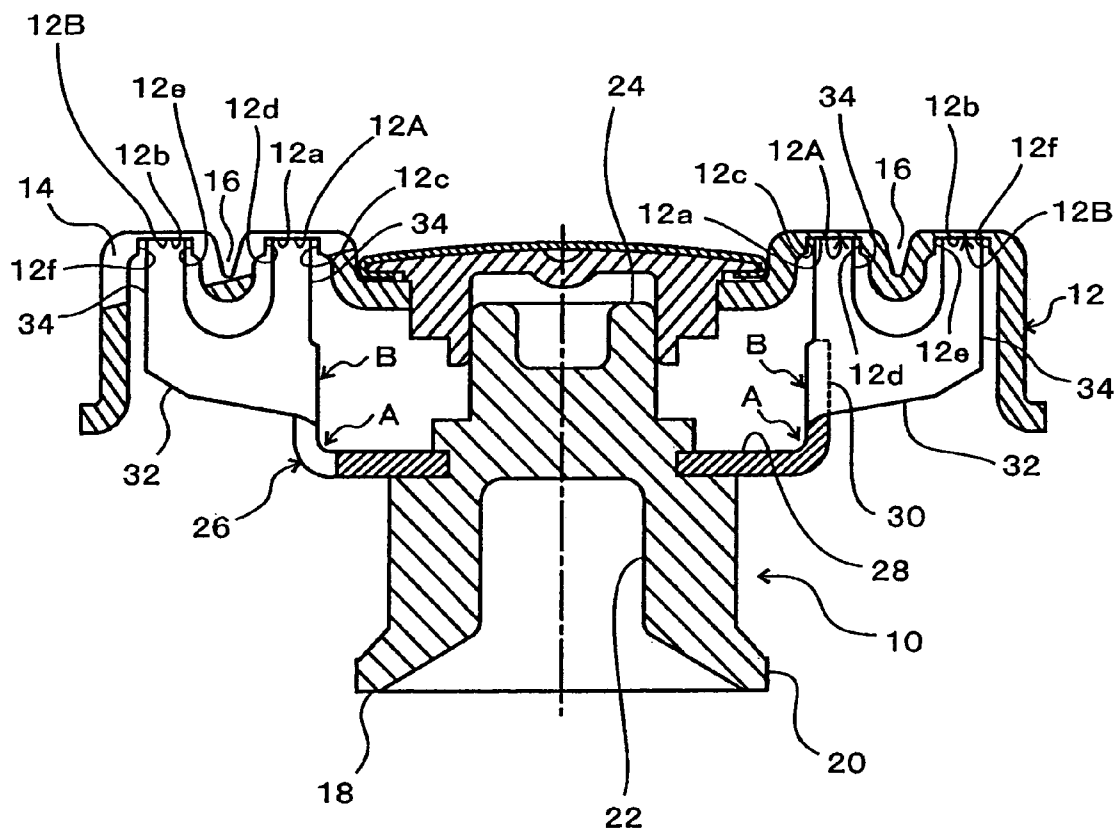
FIG. 14 PRIOR ART
