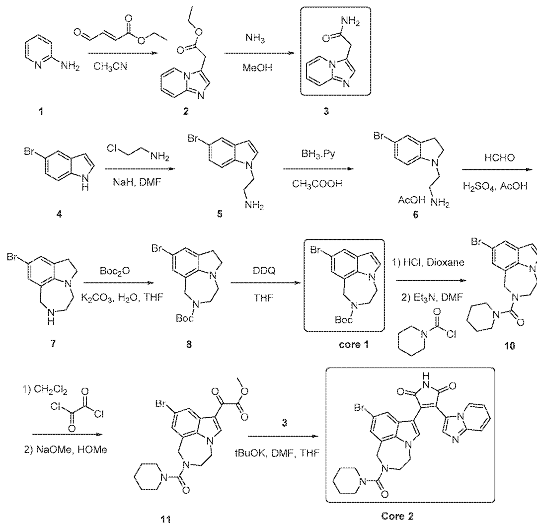
Scheme 1. General synthesis of an illustrative compound of Formula (I)
