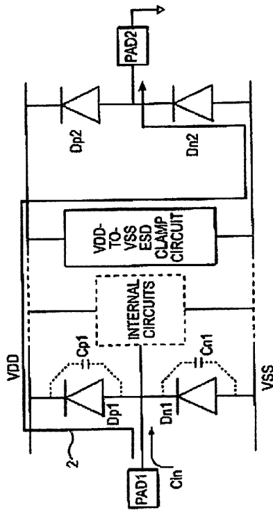
FIG. 2 PRIOR ART
