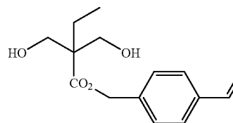
Diol Compound (3):
