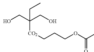
Diol Compound (2):
