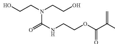
Diol Compound (3):
