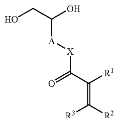
Formula (G):
