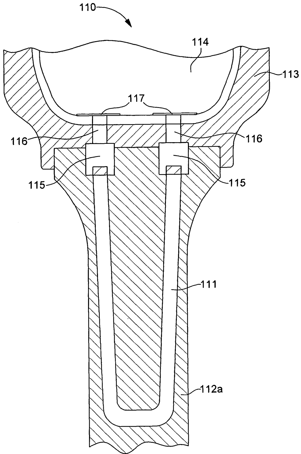
Fig. 5 ( PRIOR ART )
