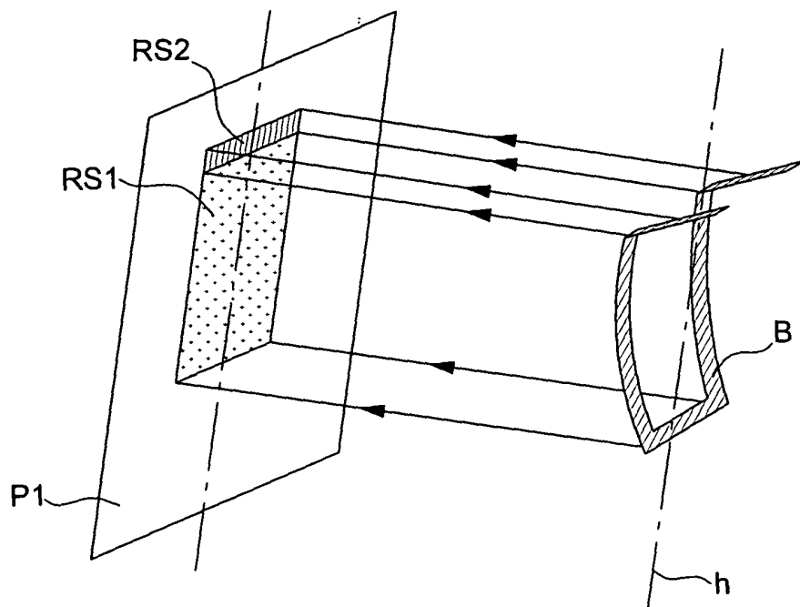
Fig. 6 (PRIOR ART)
