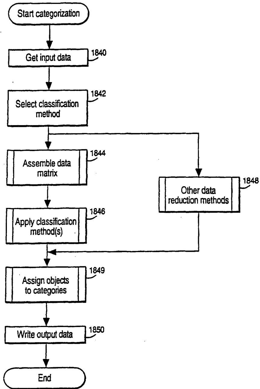
Fig. 18 Example Steps to Categorize Objects
