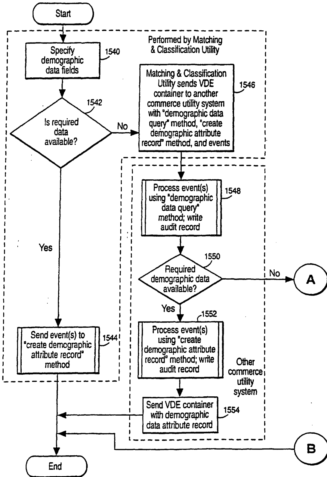
Fig. 27(A) Example Steps for Collecting Demographic Data
