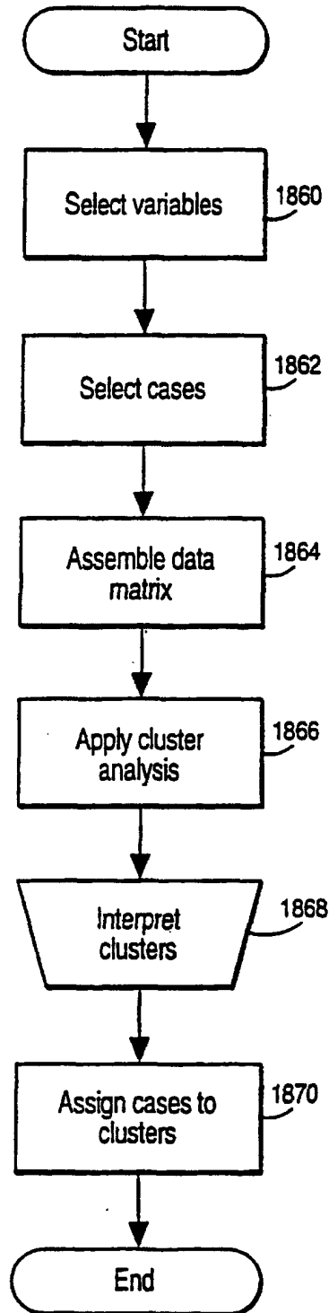
Fig. 21 Example Cluster Analysis Process
