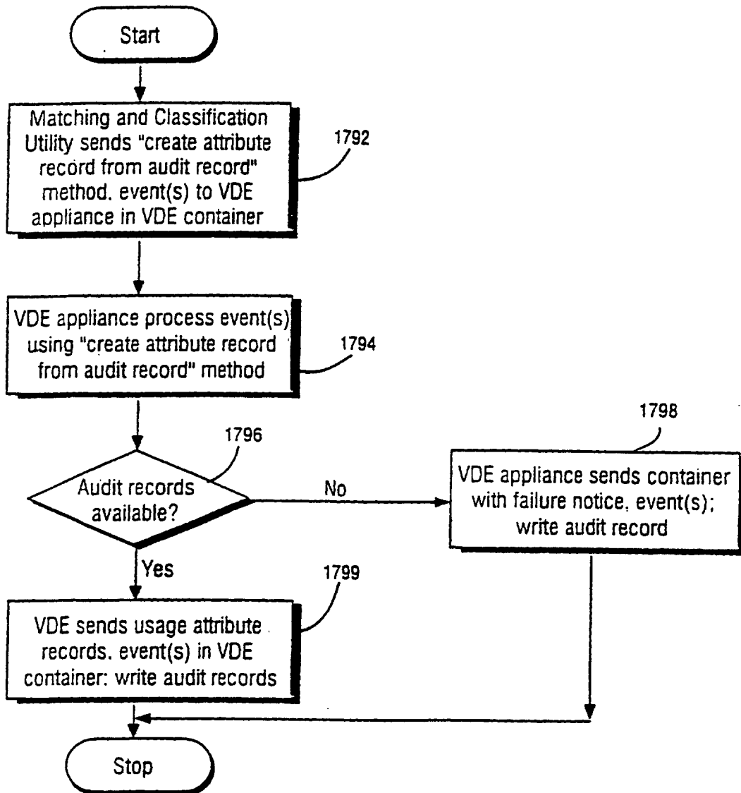
Fig. 44 Example steps for assembling usage audit records
