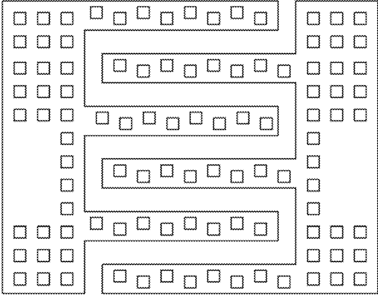
FIG. 10. Electrode pattern.
