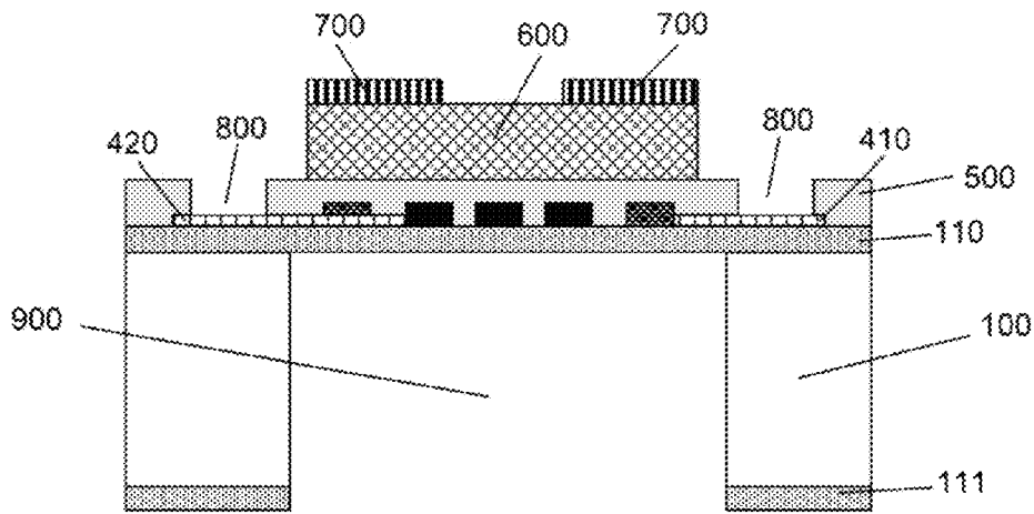
FIG. 9. Form air isolation/cavity.
