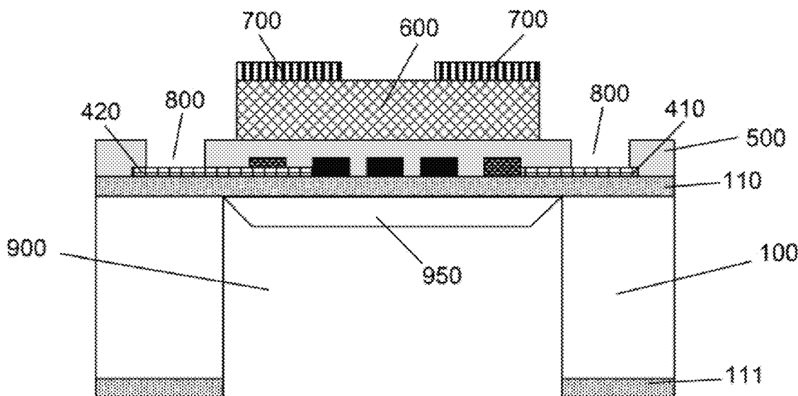
Form air isolation/cavity with a silicon plug.
