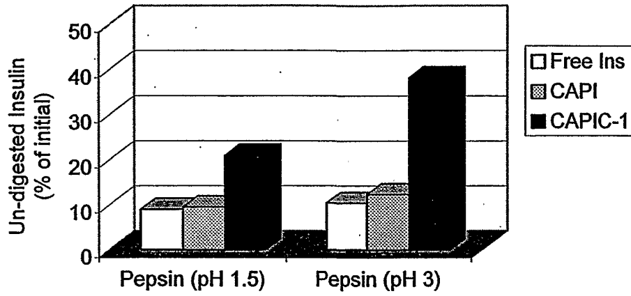
Figure 4. Stability of CAPIC oral formulation against digestive enzyme pepsin in pH 1.5 and 3 glycine buffer. 40 IU/ml insulin either free in solution, or in CAPI formulation, or CAPIC-1 formulation was incubated in 10 IU/ml pepsin for 30 min at 37C
