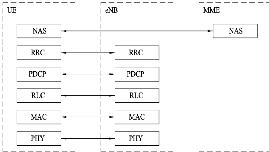
(a) Control-Plane Protocol Stack
