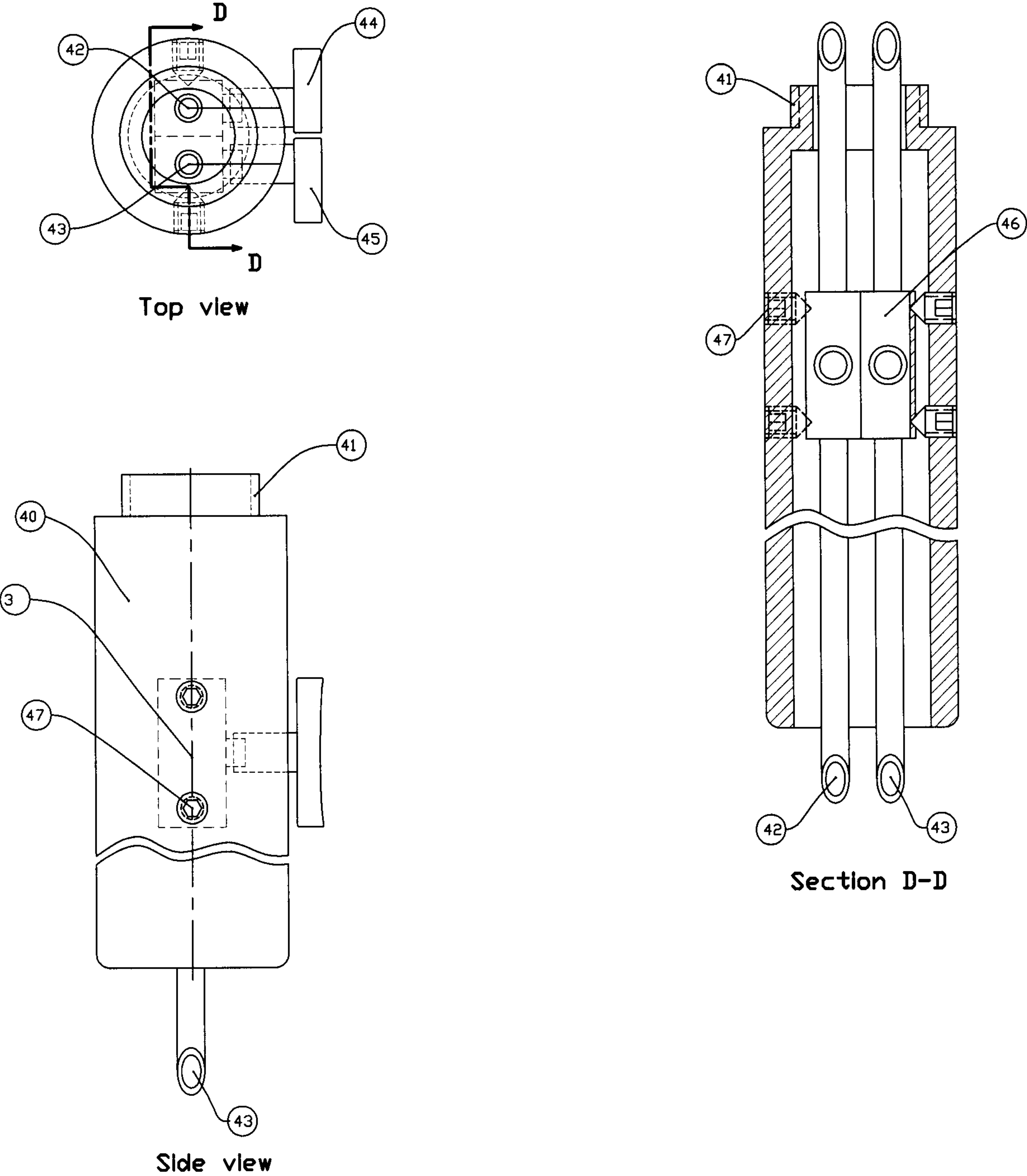
Handle
