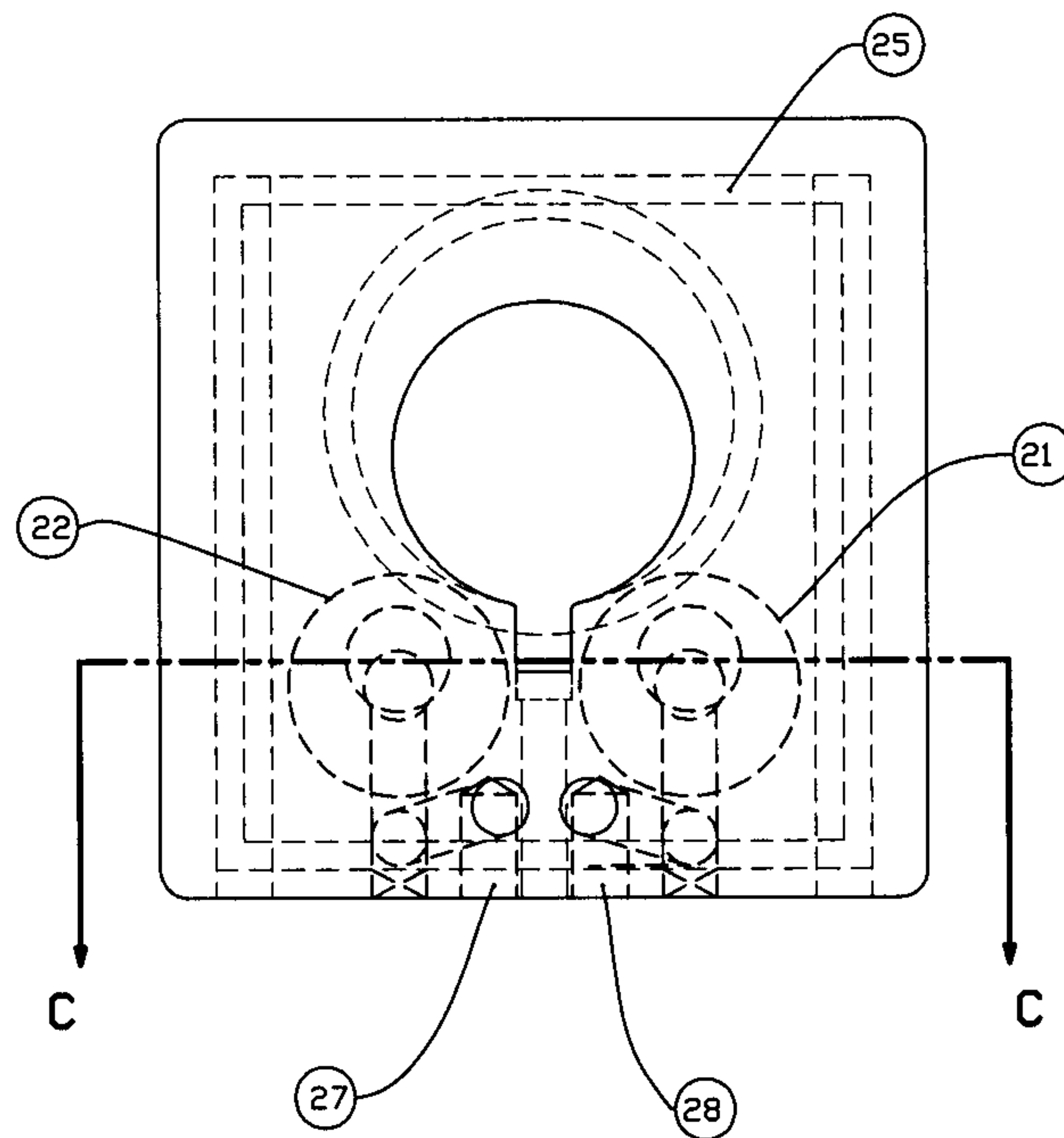
Rear Body Front View FIGURE 6
