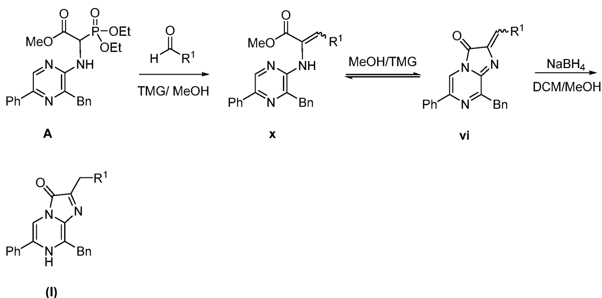
Scheme 5. Method I
