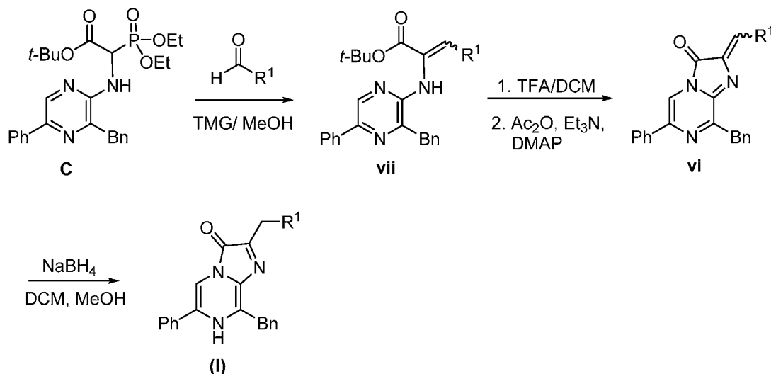
Scheme 7. Method II
