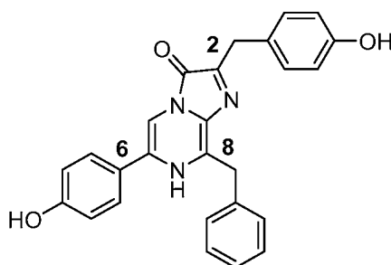
Coelenterazine
