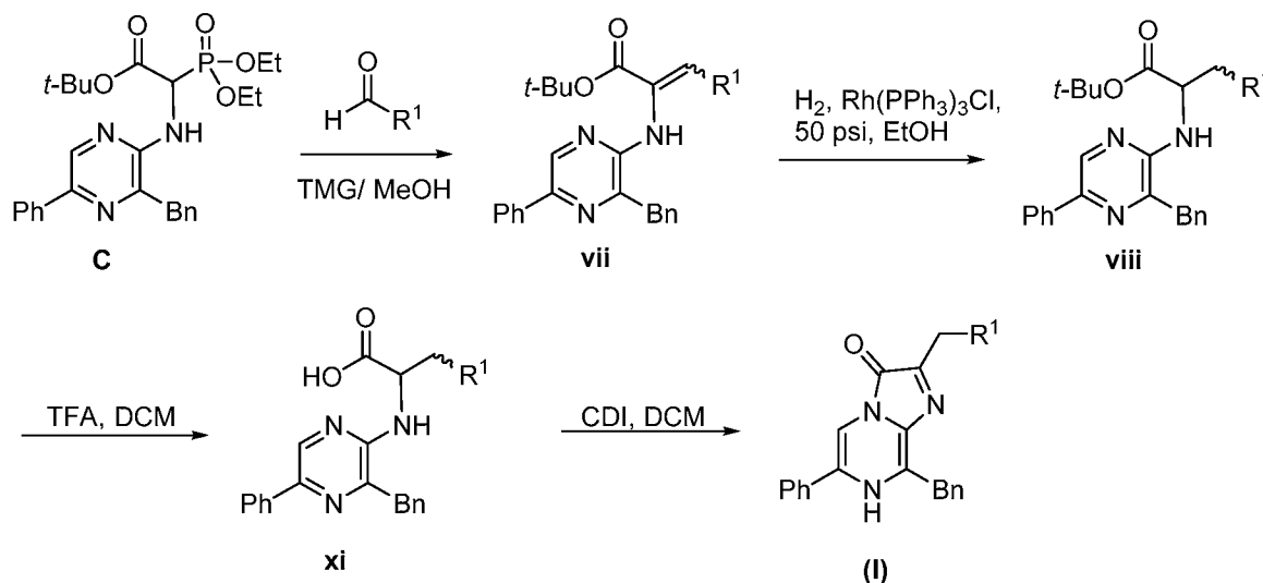
Scheme 8. Method III
