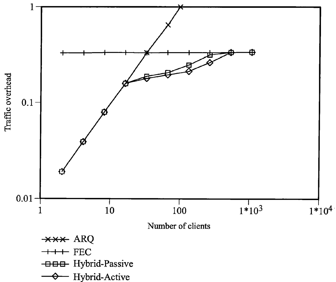
Traffic overhead versus number of receivers (packet-loss probability is 0.01).
