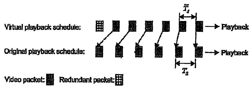
Fig. 4. Relation between the virtual playback schedule and the original schedule under FEC.
