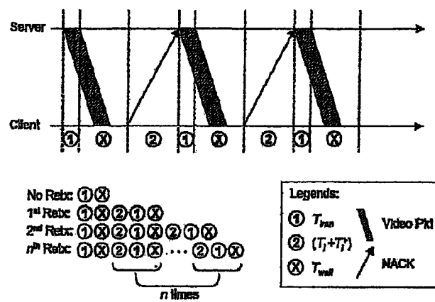
Fig. 3. Worst-case retransmission scenario for the ARQ algorithm.
