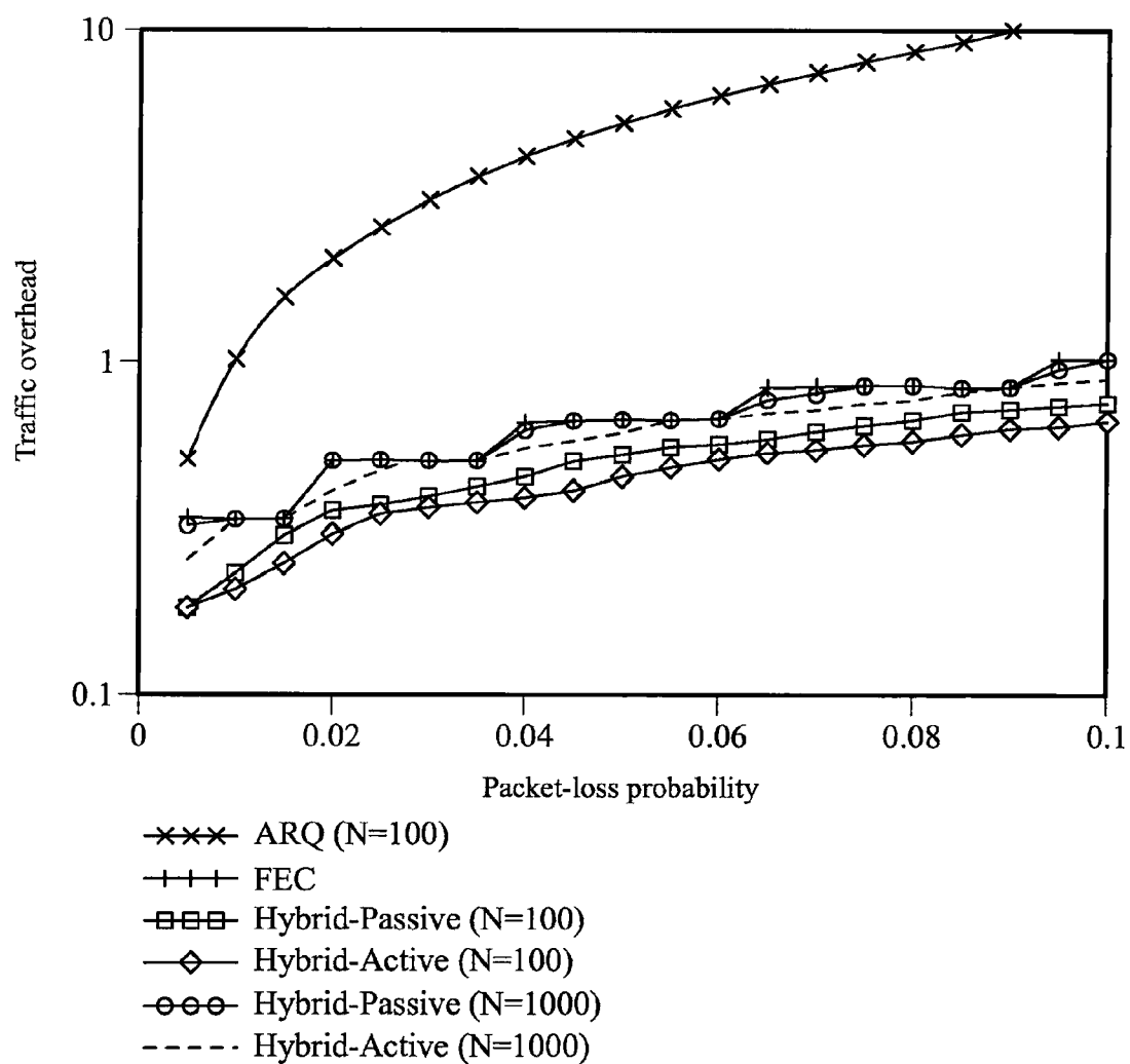
Traffic overhead versus packet-loss probability.
