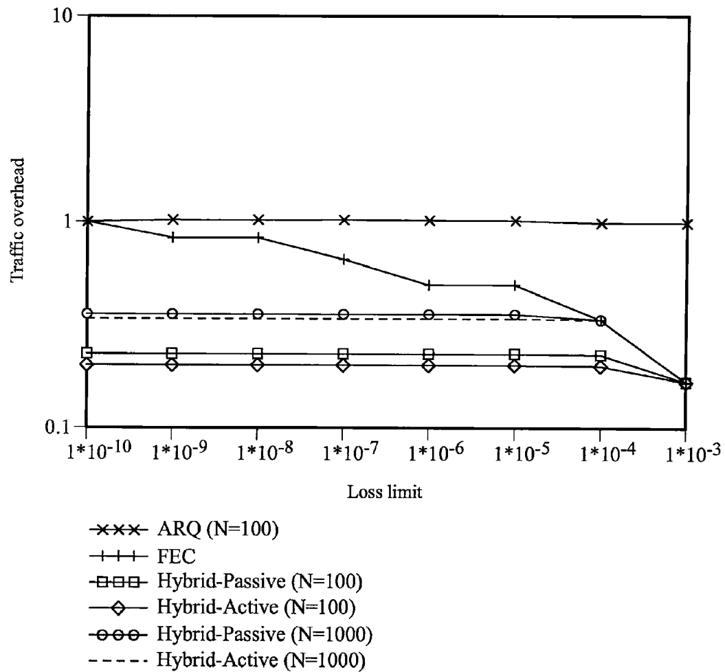
Traffic overhead versus loss limit.
