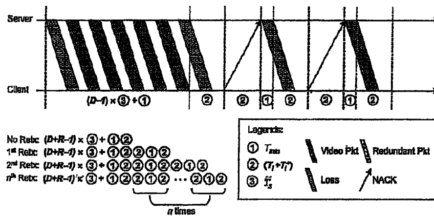
Fig. 6. Worst-case retransmission scenario for active recovery mode of the hybrid ARQ/FEC algorithm.
