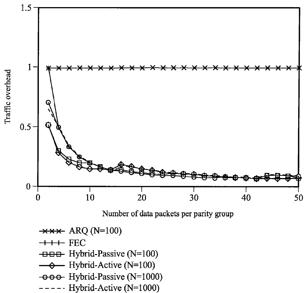
Traffic overhead versus parity group size.
