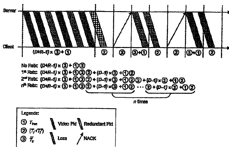
Fig. 5. Worst-case retransmission scenario for passive recovery mode of the hybrid ARQ/FEC algorithm.
