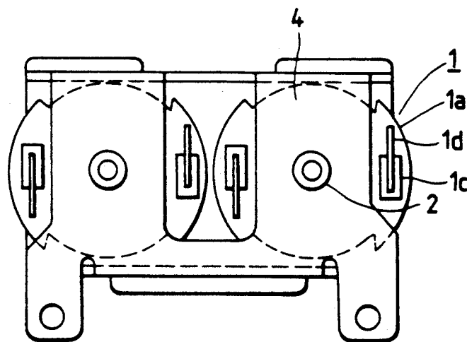
FIG. 3 PRIOR ART
