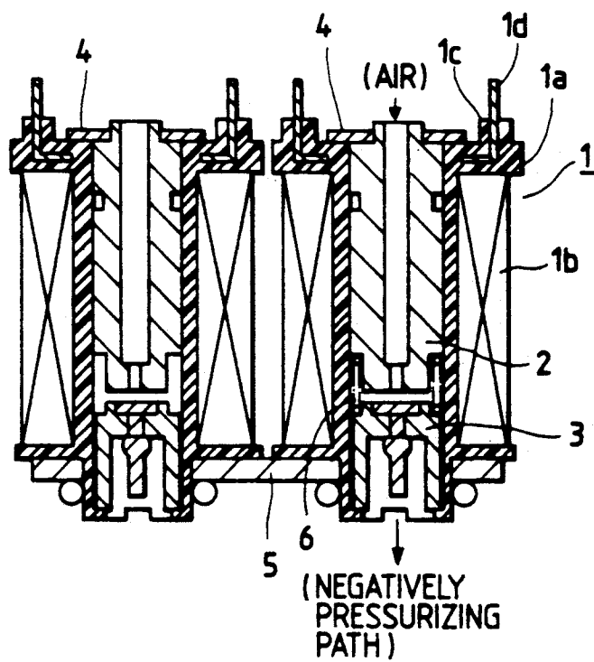
FIG. 4 PRIOR ART
