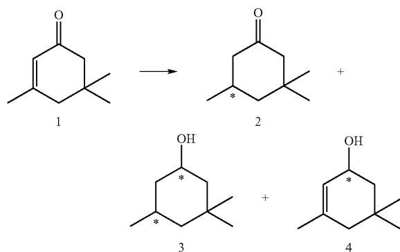
Scheme A: Asymmetric Hydrogenation of Isophorone 1
