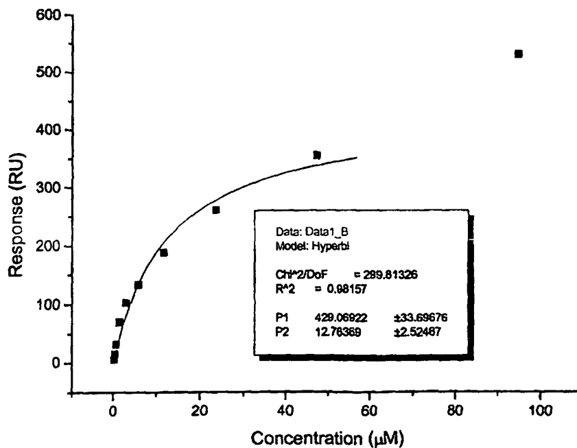
Figure 78: Thr 45/Ser 77
