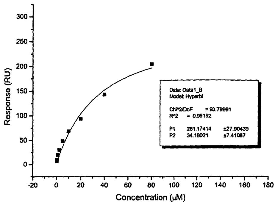
Figure 79: Tyr 10/Ser 17
