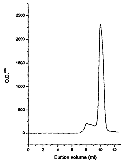
Figure 71: SEC Thr48/Ser57
