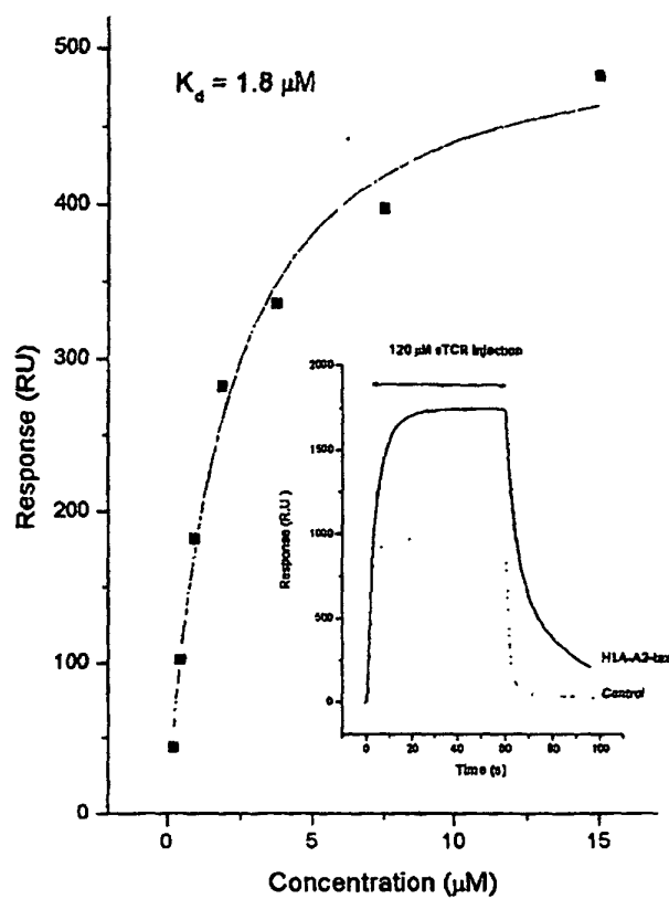
Figure 77: Thr 48/Ser 57
