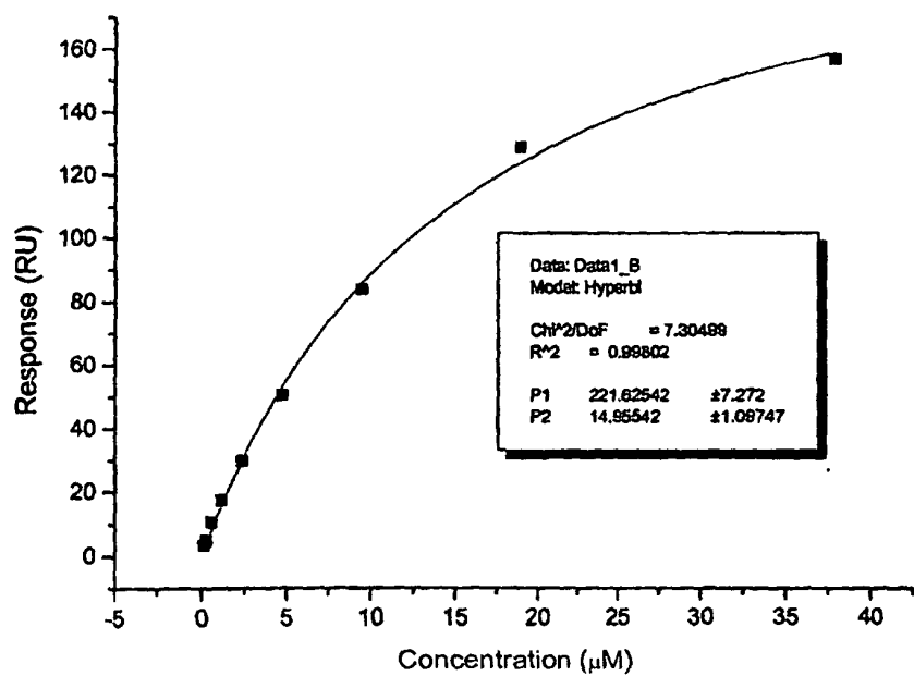
Figure 80: Thr 45/Asp 59
