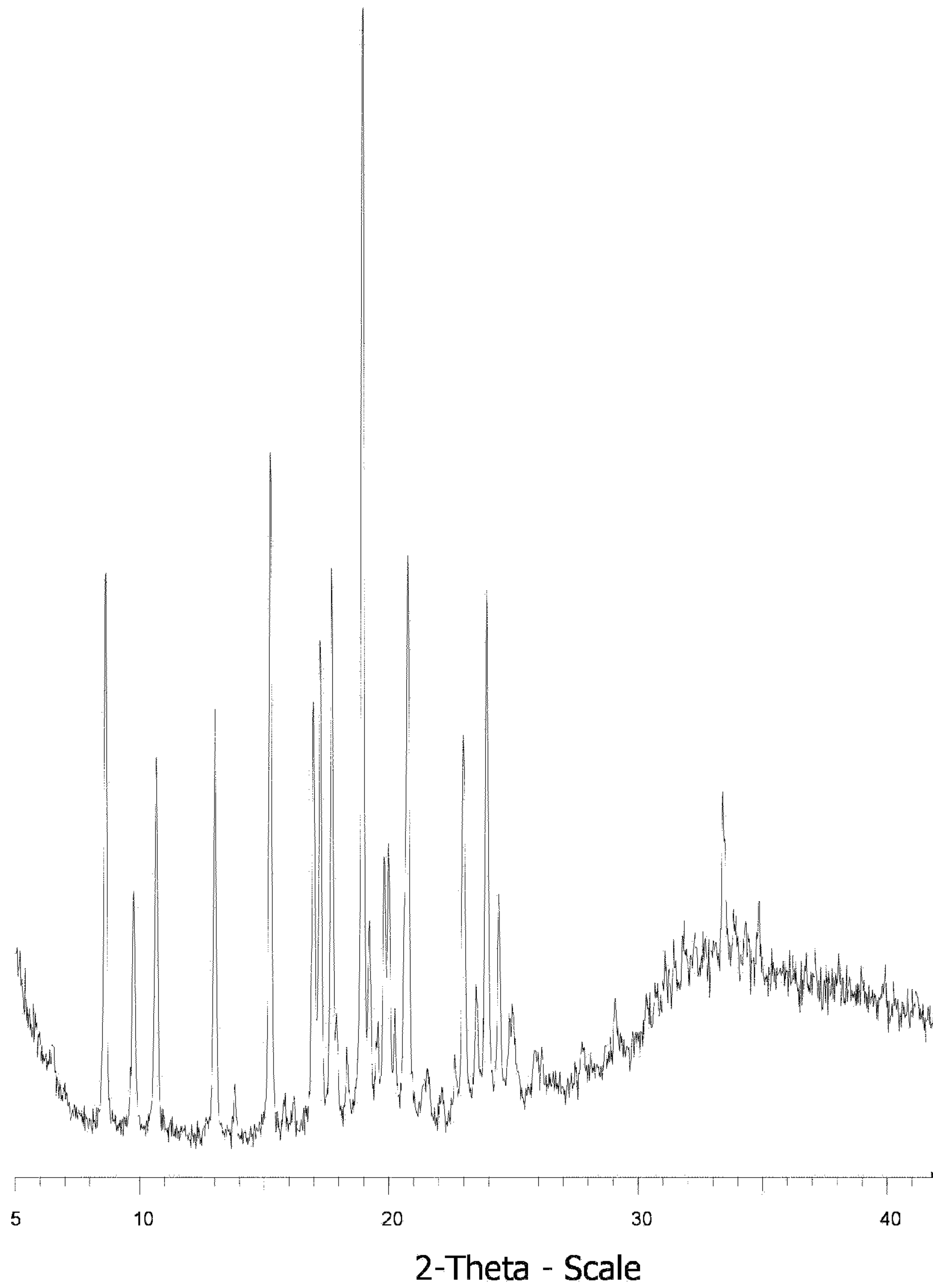
Figure 2. Compound 1 pattern 3 XRPD diffractogram
