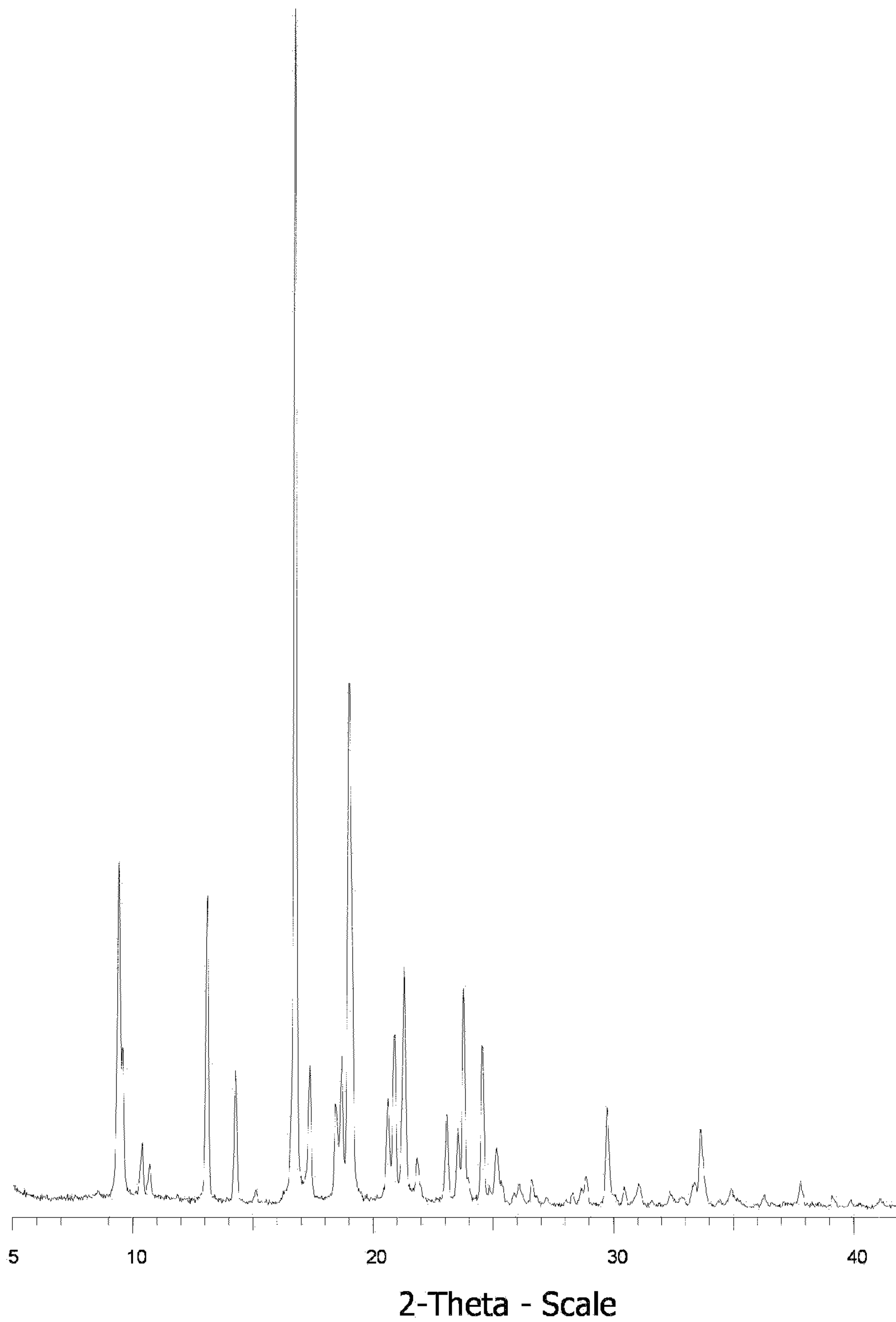
Figure 1. Compound 1 pattern 1 XRPD diffractogram
