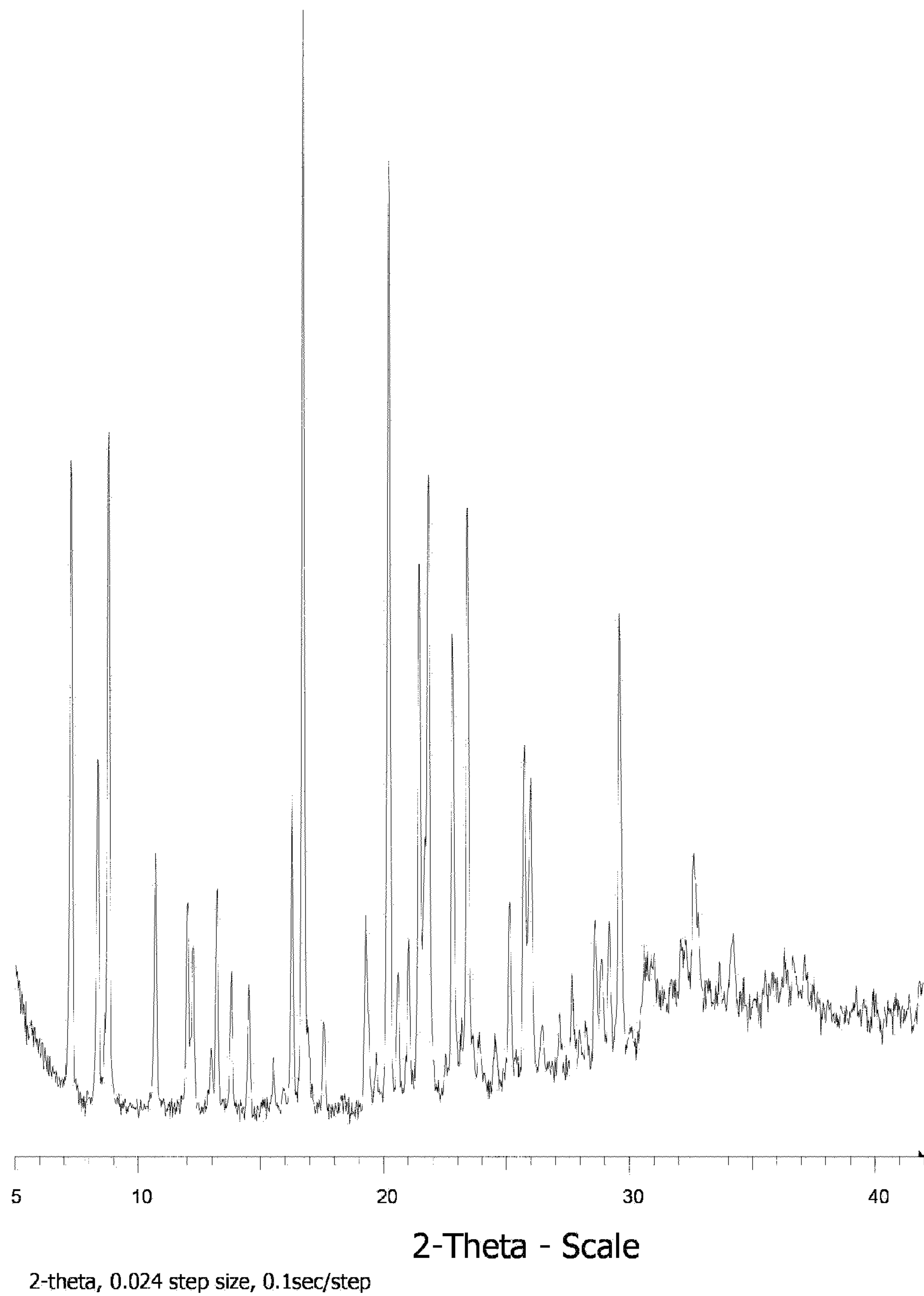
Figure 5. Compound 1, HCl.3H 2 O XRPD diffractogram
