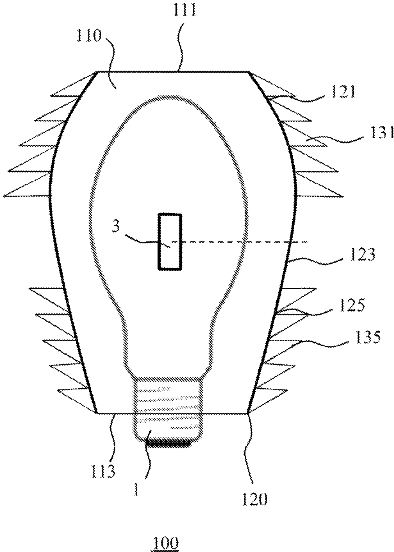
FIG. 2 (PRIOR ART)
