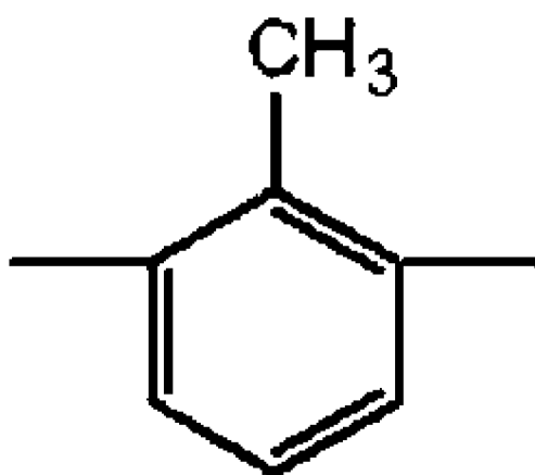
Chemical Formula (4)
