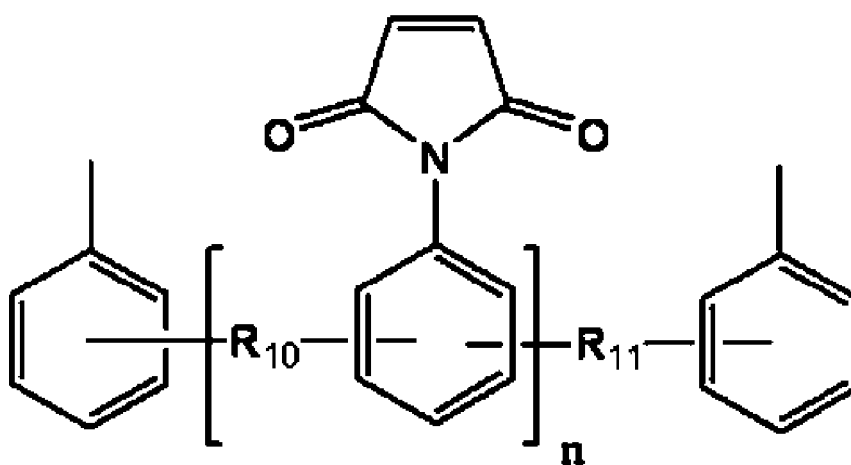
Chemical Formula (8)
