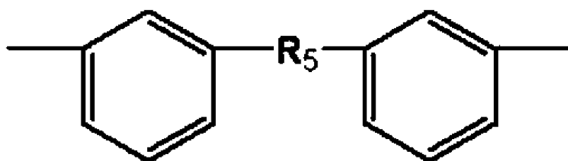
Chemical Formula (5)
