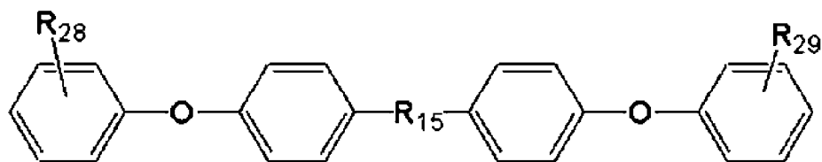
Chemical Formula (19)
