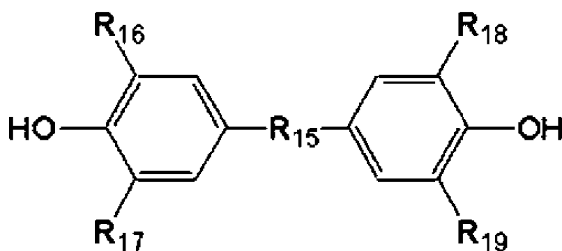
Chemical Formula (16)
