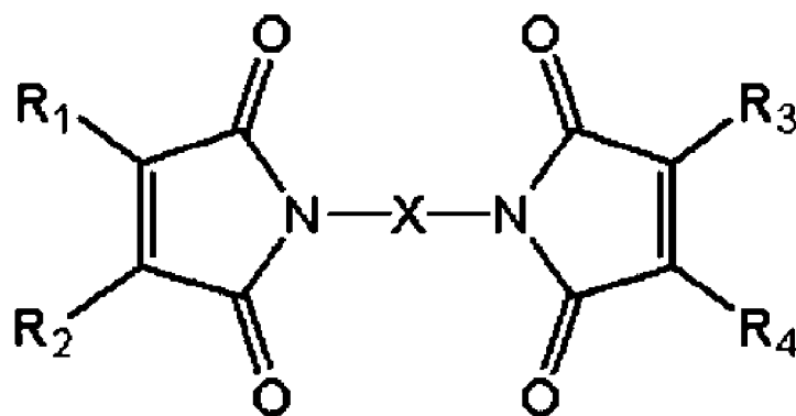
Chemical Formula (1)
