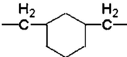
Chemical Formula (11)
