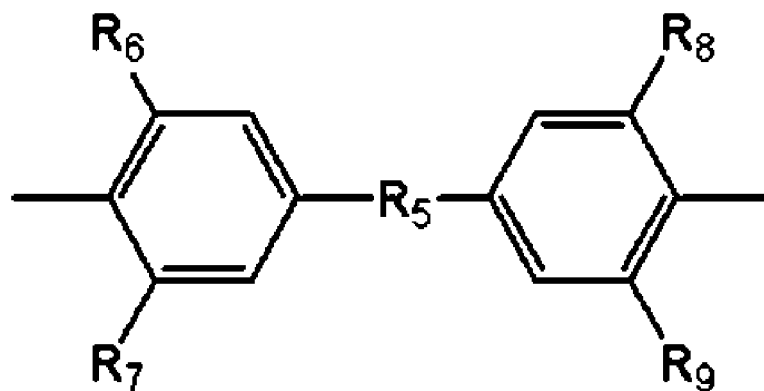
Chemical Formula (6)
