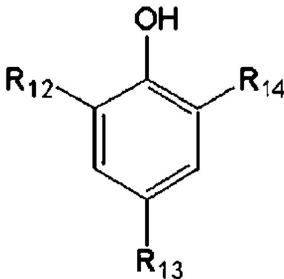
Chemical Formula (15)
