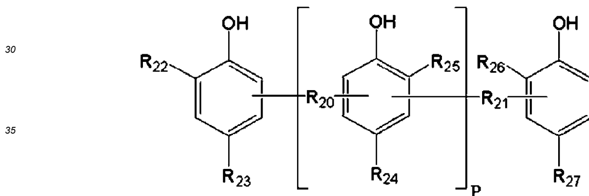
Chemical Formula (18)
