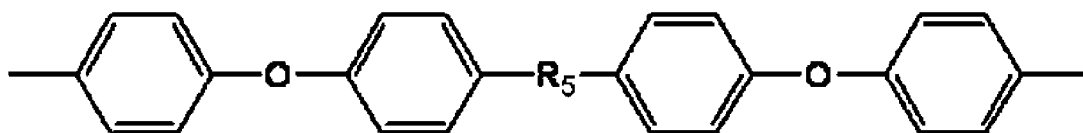
Chemical Formula (7)
