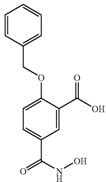
6-Benzyloxy-N-hydroxy-isophthalamic acid
