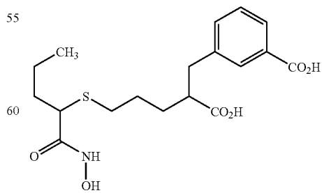
3-[2-Carboxy-5-(1-hydroxycarbonylbutylsulfanyl)-pentyl]-benzoic acid
