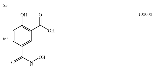
6,N-Dihydroxy-isophthalamic acid
