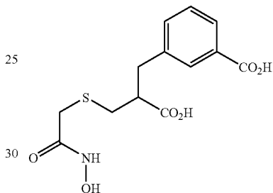
3-(2-Carboxy-3-hydroxycarbonylmethylsulfanyl)propyl)-benzoic acid
