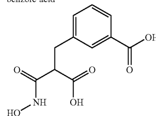
3-(2-Carboxy-2-hydroxycarbamoyl-ethyl)-benzoic acid
