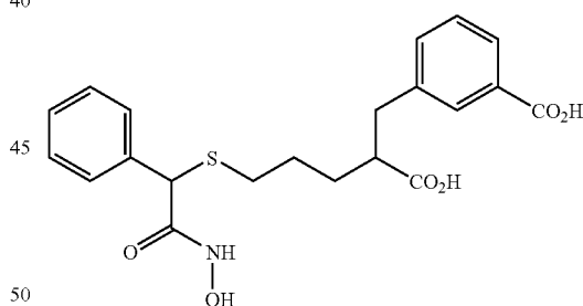
3-[2-Carboxy-5-(hydroxycarbonylphenylmethylsulfanyl)-pentyl]-benzoic acid
