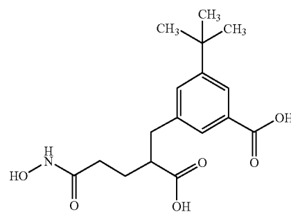
3-tert-Butyl-5-(2-carboxy-4-hydroxycarbamoyl-butyl)-benzoic acid
