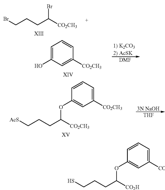
SCHEME VII
