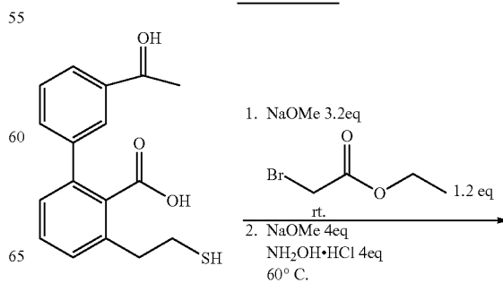
SCHEME XV
