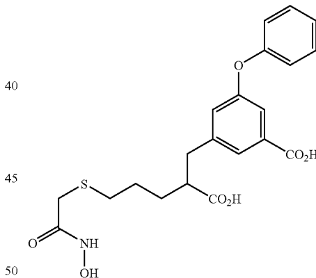
3-(2-Carboxy-5-hydroxycarbonylmethylsulfanyl)pentyl)-5-phenoxy-benzoic acid
