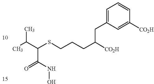
3-[2-Carboxy-5-(1-hydroxycarbonyl-2-methyl-propylsulfanyl)-pentyl]-benzoic acid
