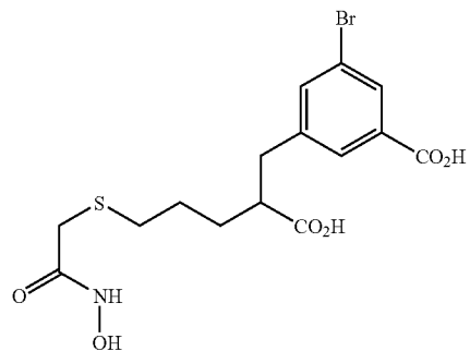
3-Bromo-5-(2-carboxy-5-hydroxycarbonylmethylsulfanyl)pentyl)-benzoic acid
