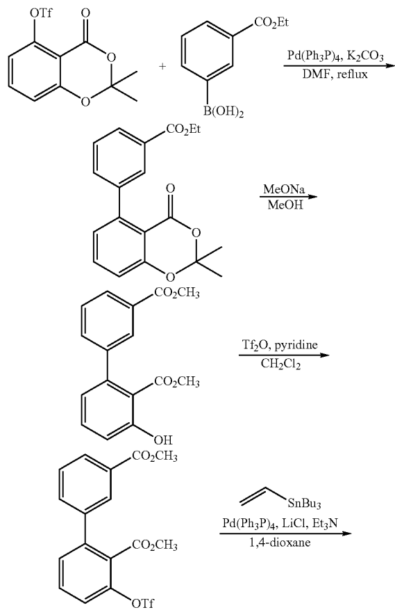
SCHEME VIII
