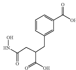
3-(2-Carboxy-3-hydroxycarbamoyl-propyl)-benzoic acid
