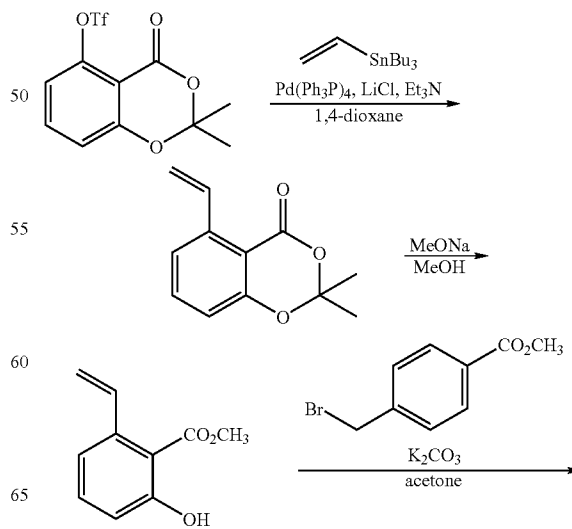
SCHEME IX
