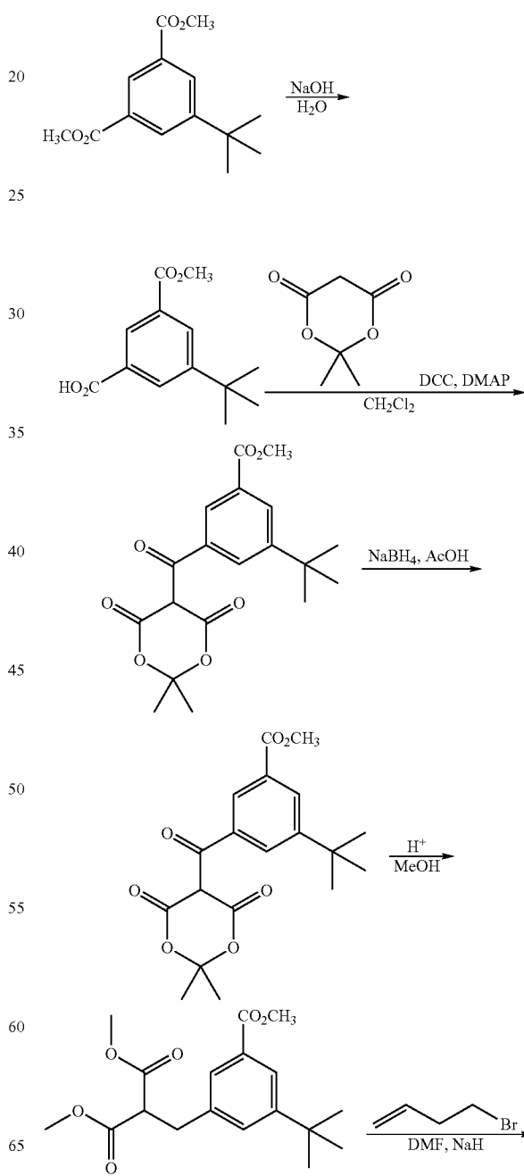
SCHEME XI
