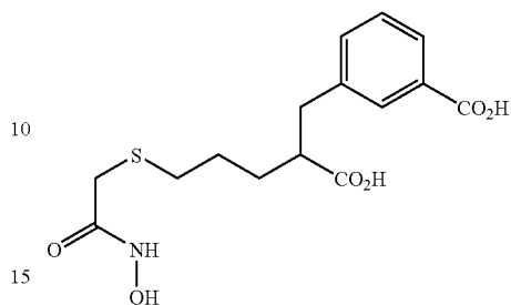
3-(2-Carboxy-5-hydroxycarbonylmethyl-
