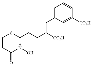
3-[2-Carboxy-5-(2-hydroxycarbonylmethyl-ethylsulfanyl)-pentyl]-benzoic acid
