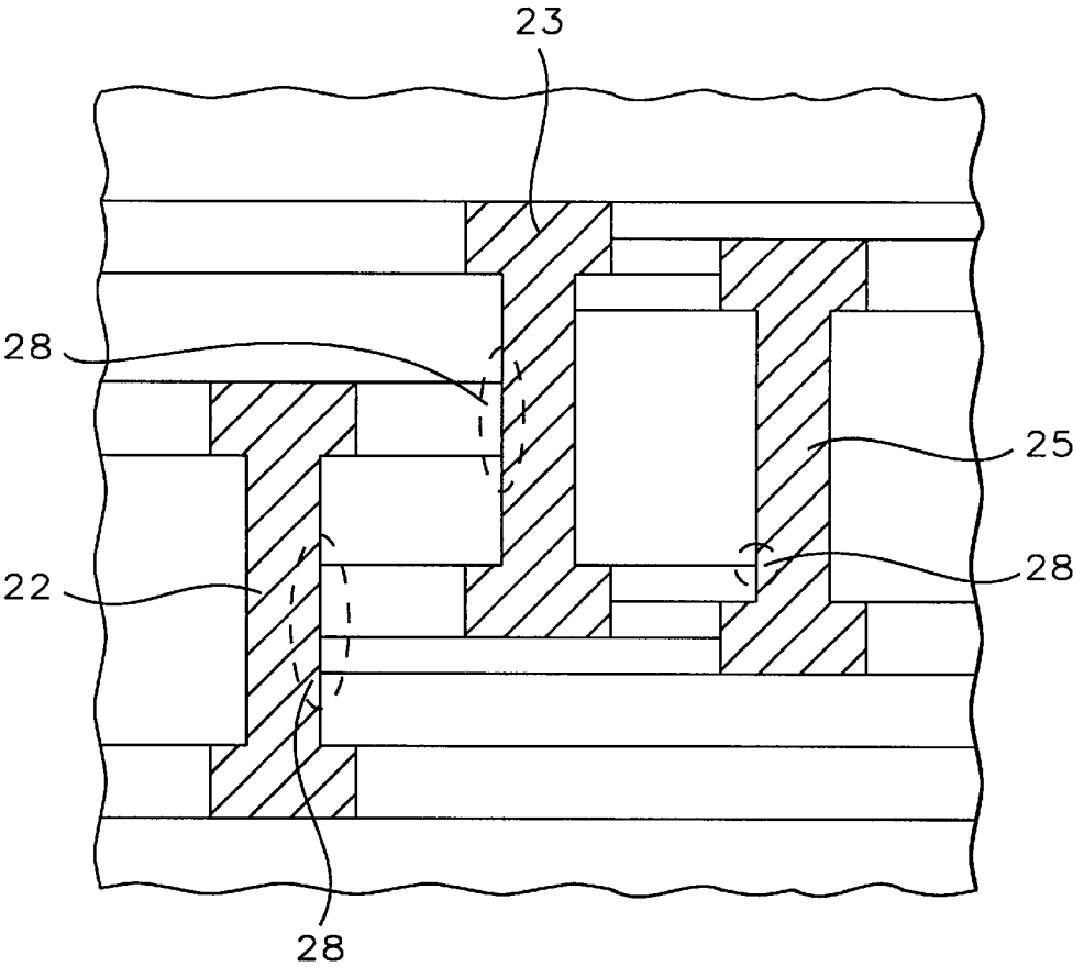
FIG. 2 - Prior Art
