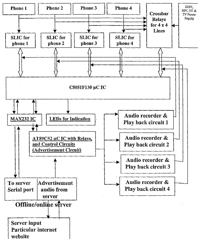
BLOCK DIAGRAM OF THE PHONE EXCHANGE WITH ADVERTISEMENT PLAYER AND NEW PROCESS CIRCUIT
