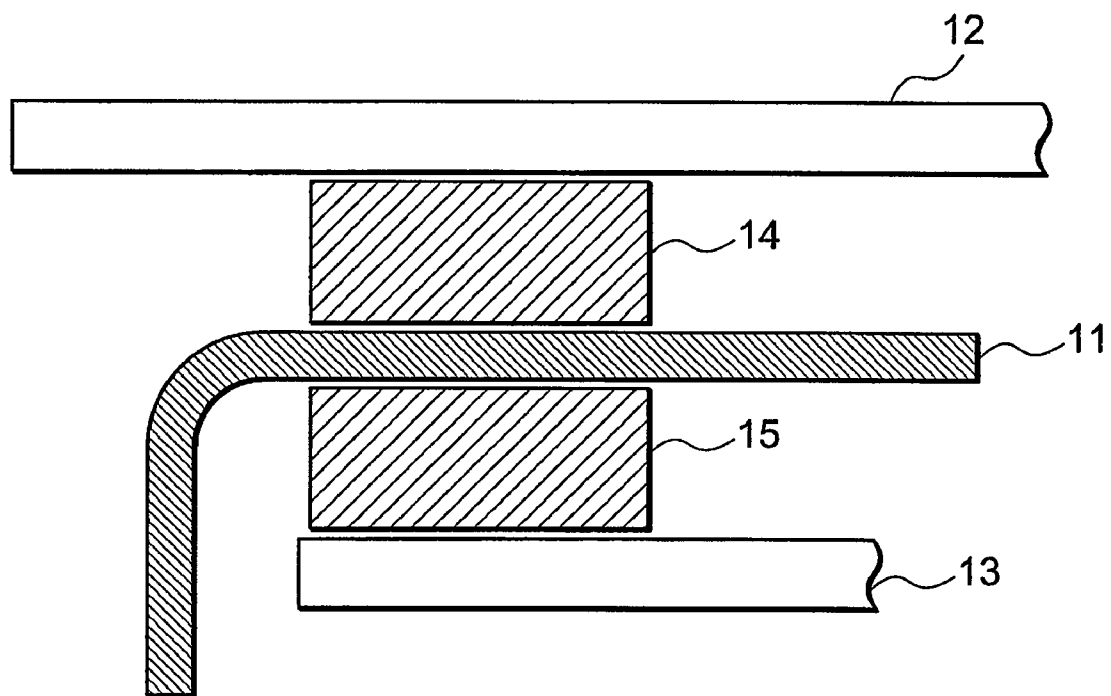
FIG. 1 (RELATED ART)
