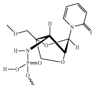
2',4'-BNA-2-pyridone
