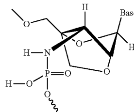
2',4'-ENA
