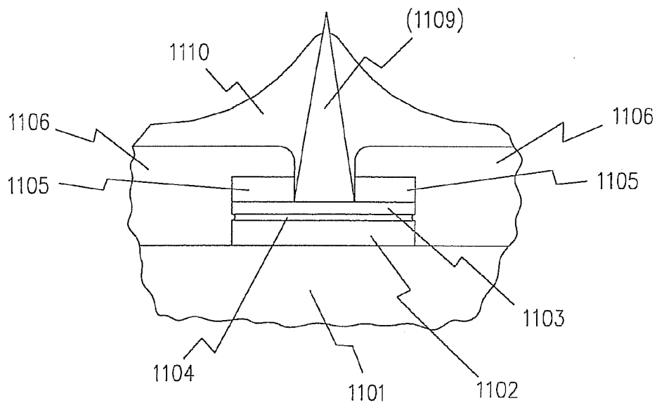
FIGURE 11b ELECTRODES
