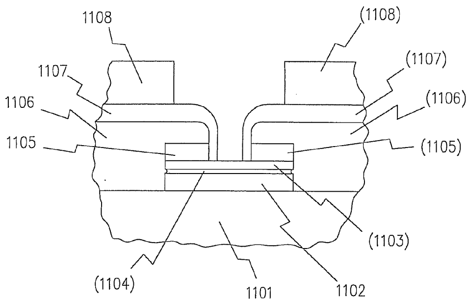
FIGURE 11a ELECTRODES
