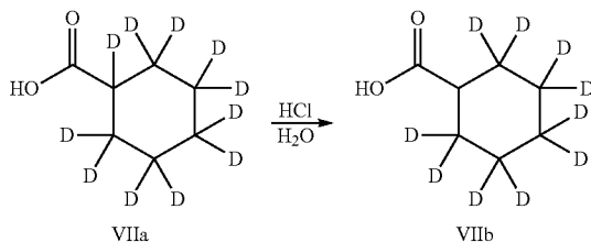
Scheme 2: Method for Preparation of Intermediate VIIb
