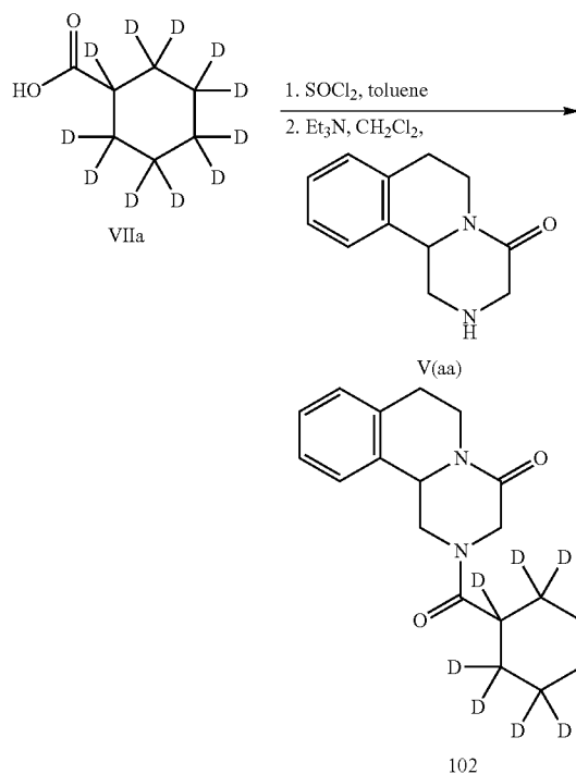
Scheme 11. Preparation of Compound 102
