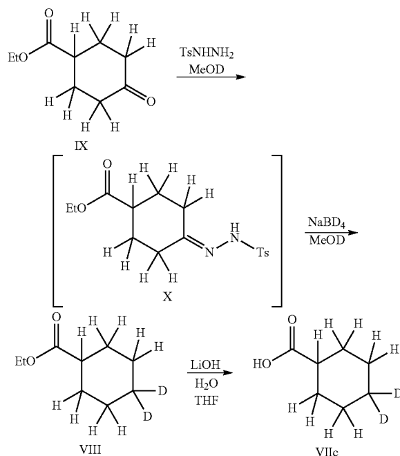
Scheme 7. Preparation of Intermediate VIIc
