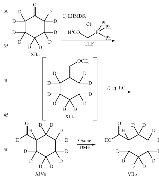
Scheme 6a. Preparation of Intermediate VIIb
