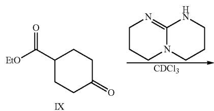
Scheme 4: Method for Preparation of Intermediate VIId:
