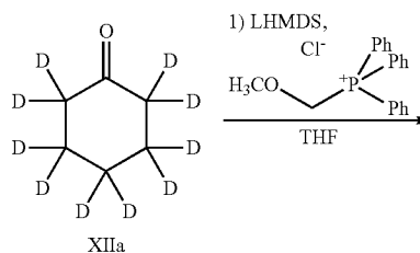
Scheme 2b: Alternative Method for Preparation of Intermediate VIIb:
