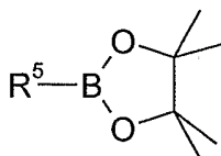
Formula 9b
