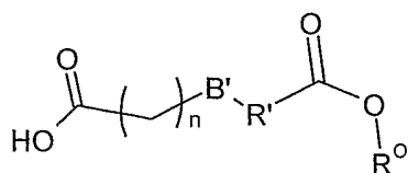
Formula 6b'
