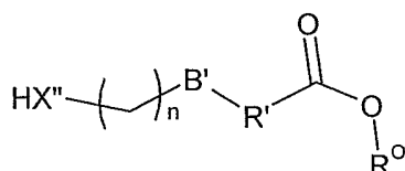
Formula 6b"
