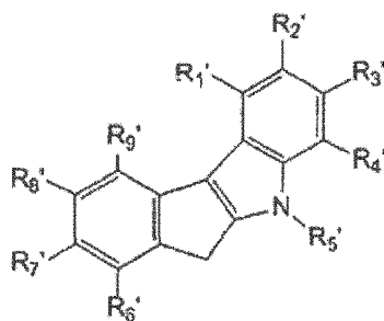
[Chemical Formula 2c]
