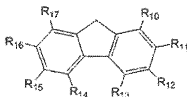
[Chemical Formula 2c]
