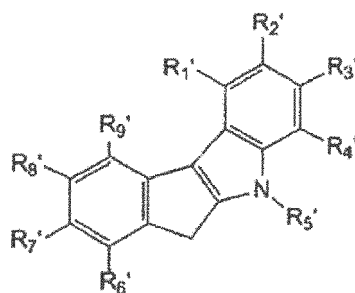
[Chemical Formula 2b]
