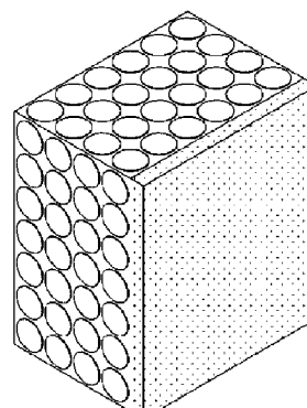
Attach a Copper Collector to Lithium-Filled Porous Structure
