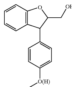
Chemical Formula
