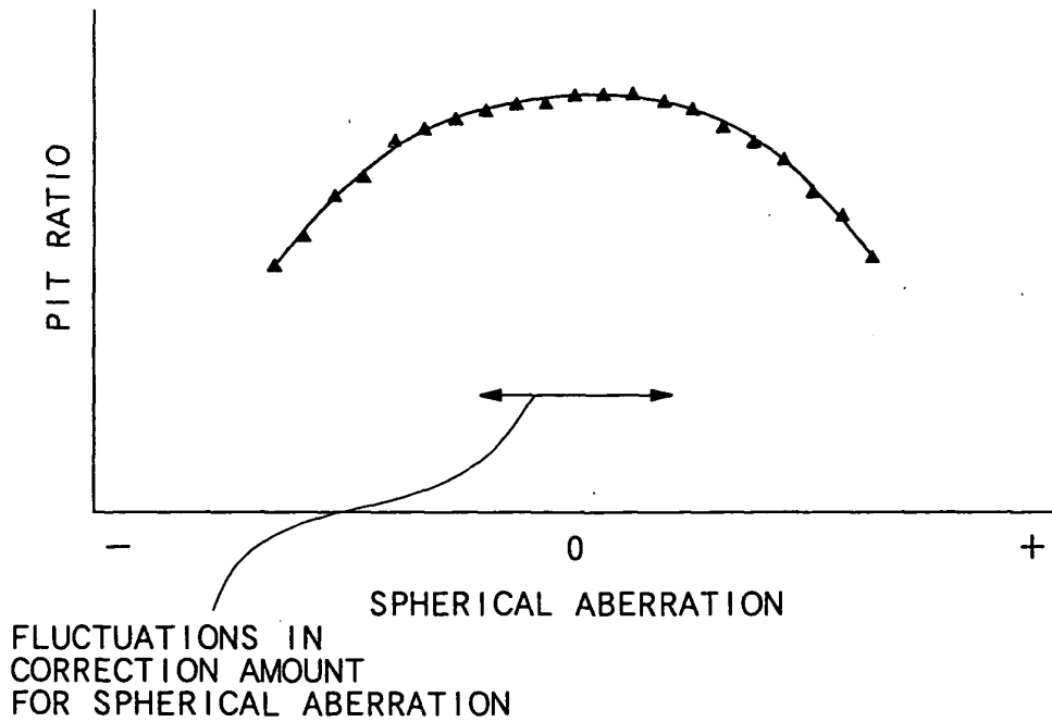
DVD-R SPHERICAL ABERRATION VS PIT RATIO
