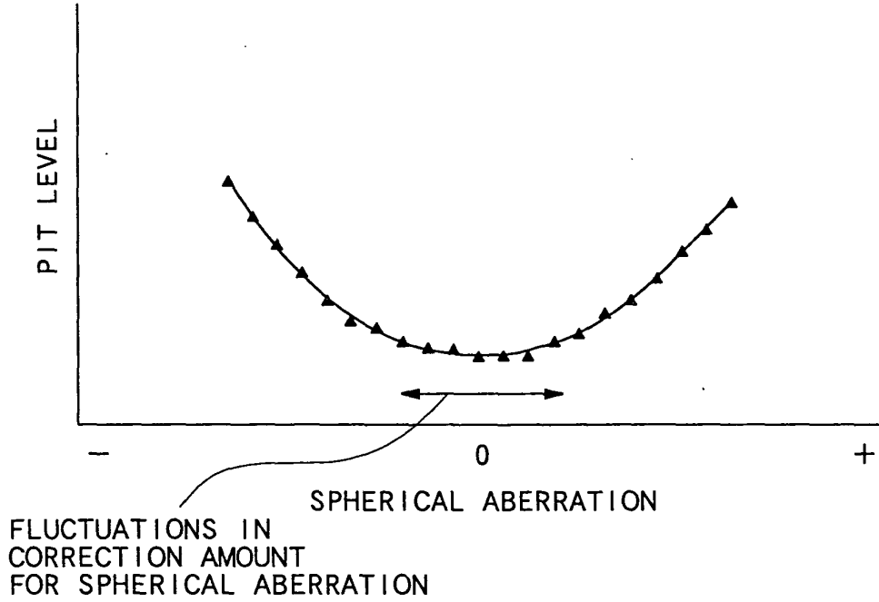
DVD-R SPHERICAL ABERRATION VS PIT LEVEL
