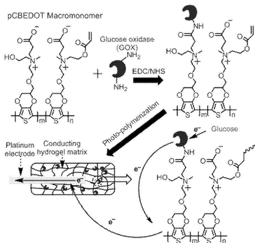
Fig. 13. Illustration of pCBEDOT glucose sensor.
