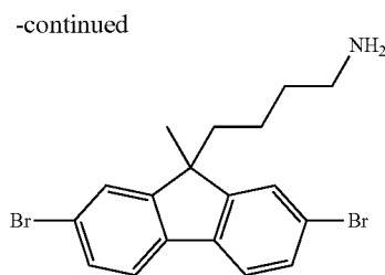
Step 3: 4-(2,7-dibromo-9-methyl-9H-fluoren-9-yl)butan-1-amine
