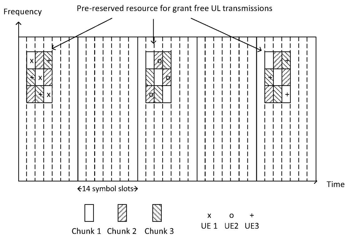
Figure 2 – Conventional resource allocation for grant free UL, single UE per resource chunk with frequency hopping, GF opportunity every 2 slots, K=3
