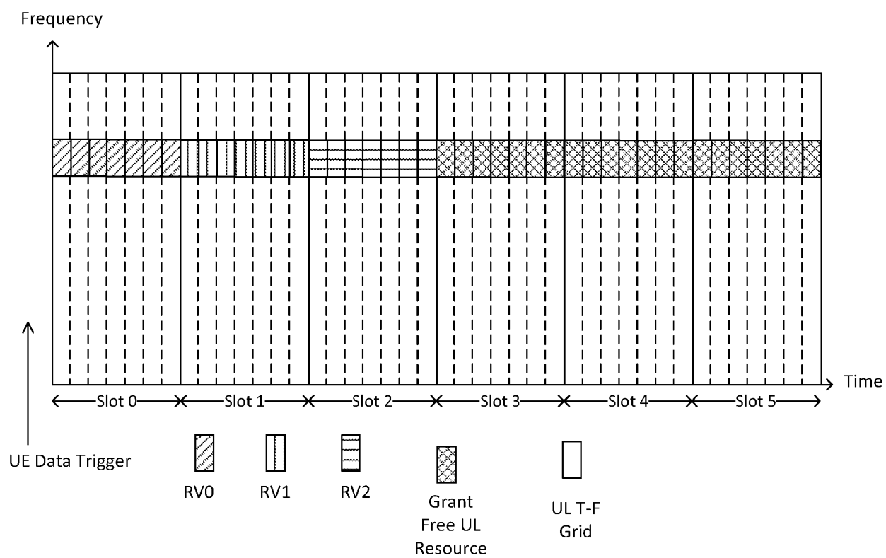
Figure 5: RV association to GF occasion
