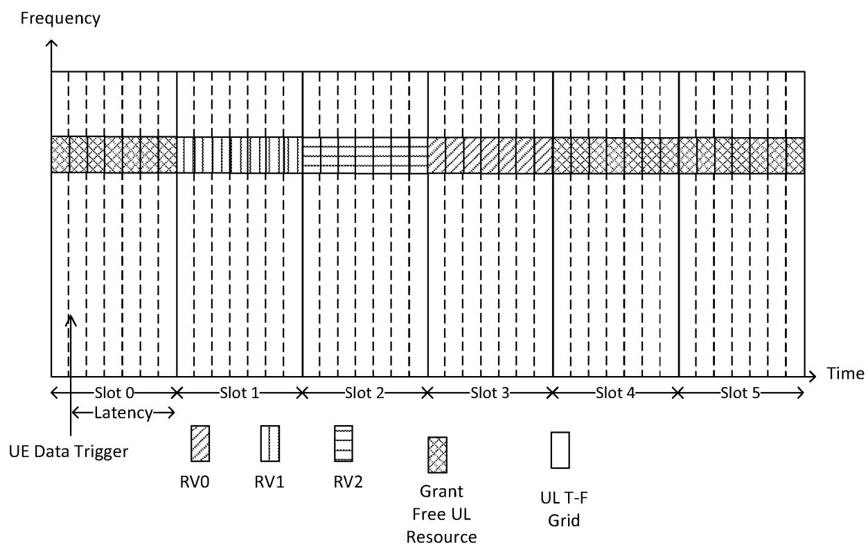
Figure 7 : Proposal for RV association to GF transmission occasions
