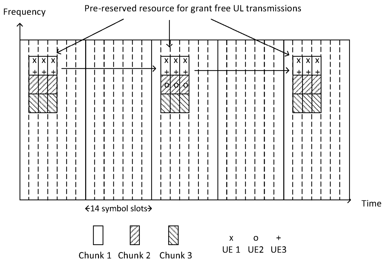
Figure 3- Multi UEs allocation per resource chunk
