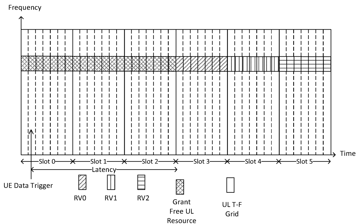
Figure 6: RV association to FG occasion – Problem with conventional approach
