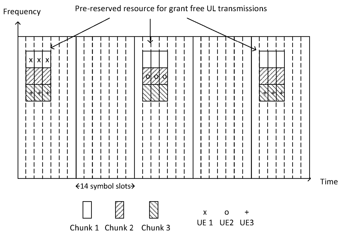
Figure 1 – Conventional resource allocation for grant free UL, single UE per resource chunk, GF opportunity every 2 slots, K=3
