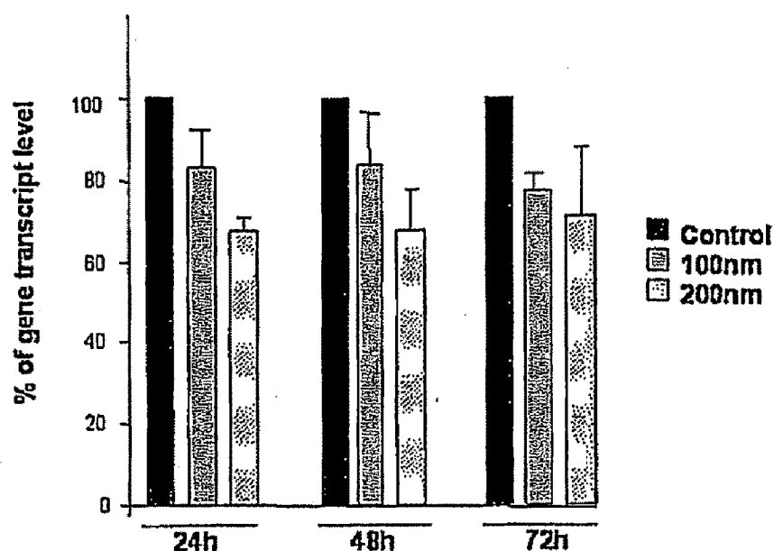
Figure 4. Time-dose response of siRNA in the P2RX7 downregulation. The values represent the mean expression level of P2RX7 transcript at different siRNA2 (targeting the murine sequence homologous to human SEQ. ID. 78) time (24, 48 and 72h) and dose treatments (100 and 200 nm). The samples were analyzed by Real-time PCR and normalized using actin as the reference housekeeping gene.
