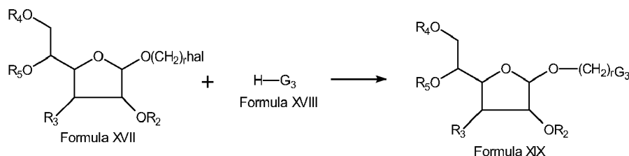
Scheme V
