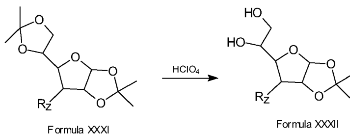
SCHEME VIII
