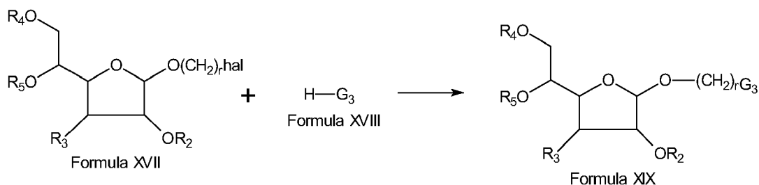
Scheme V
