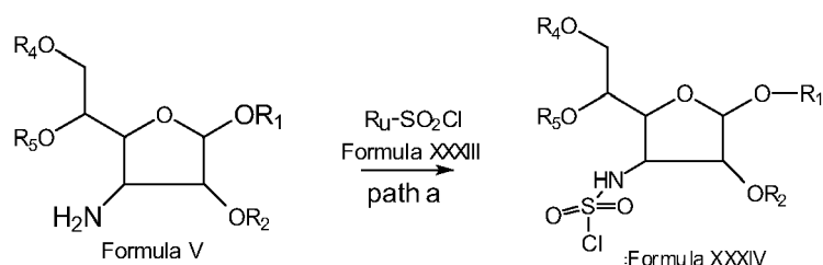
SCHEME IX
