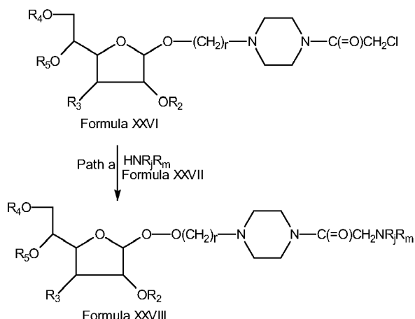
SCHEME VII
