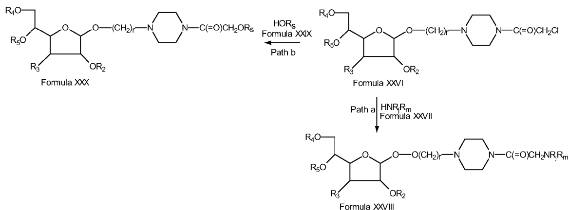
SCHEME VII
