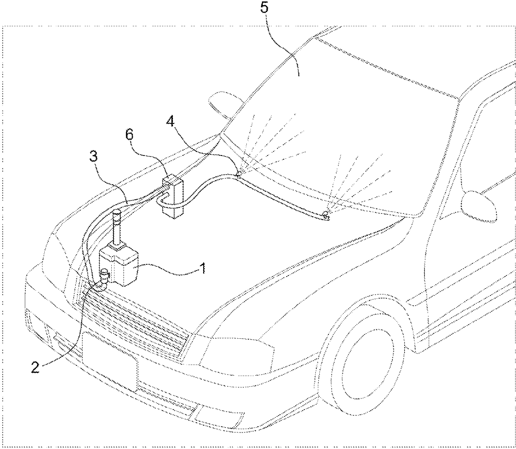
FIG. 2 (Related Art)
