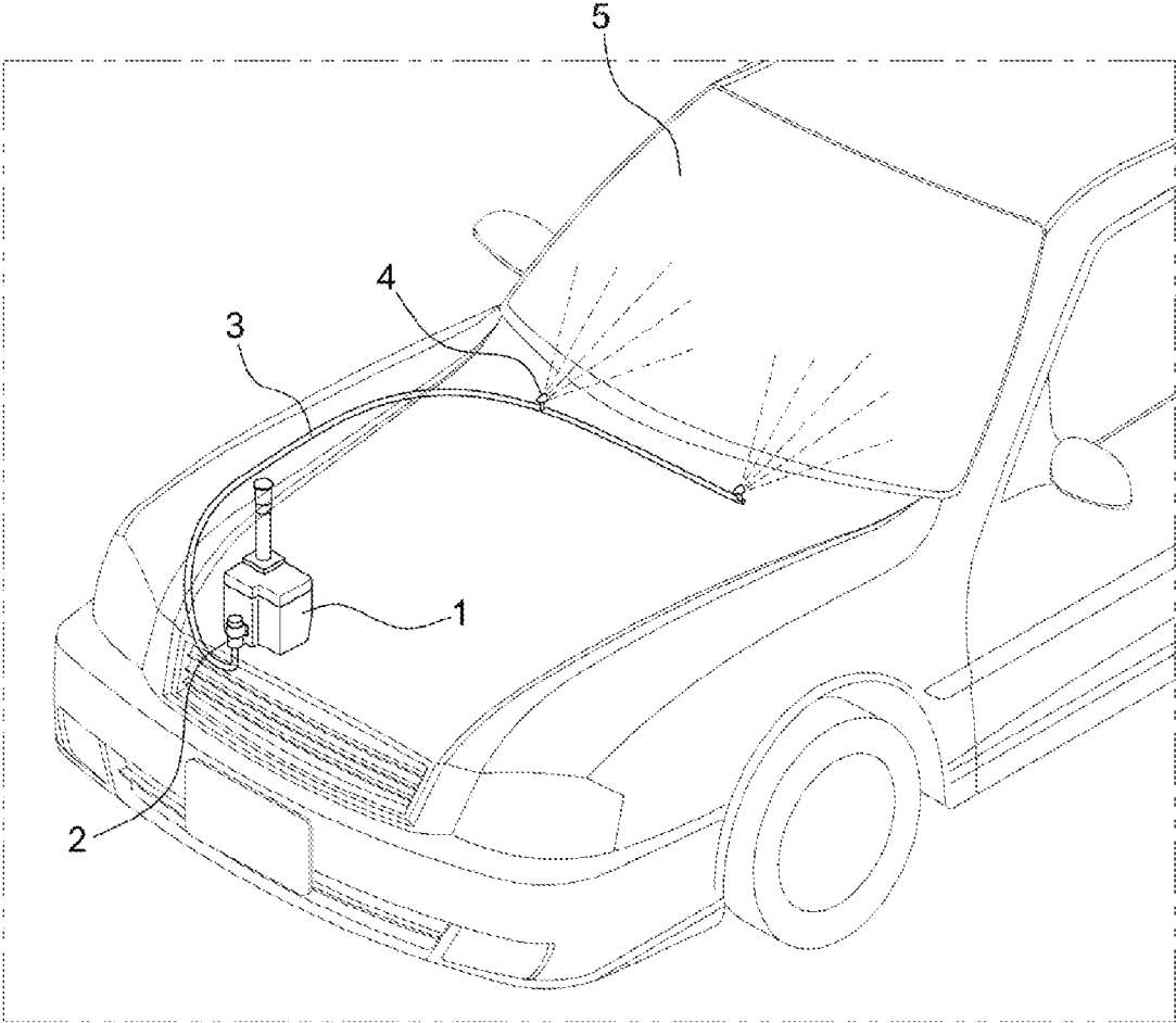
FIG. 1 (Related Art)
