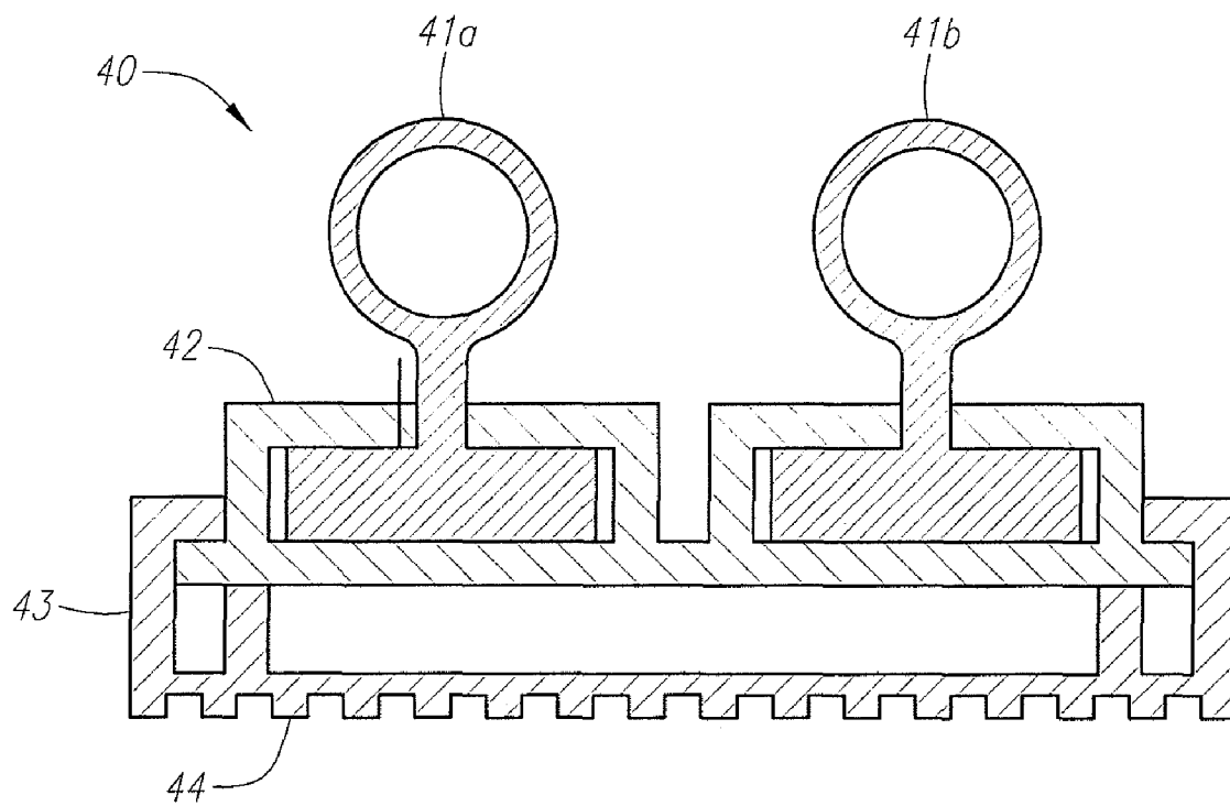
FIG. 4 (PRIOR ART)
