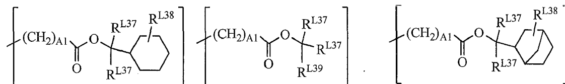
(A-1)-7
