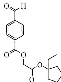
Aldehyde 6
