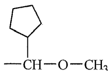
(A-2)-41
