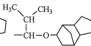
(A-2)-57
