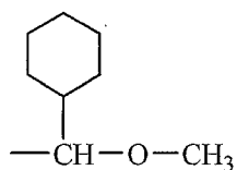
(A-2)-40
