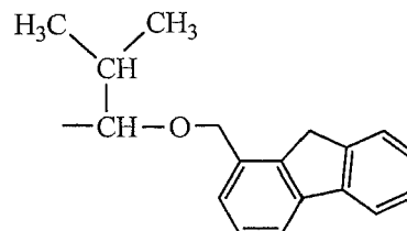
(A-2)-66
