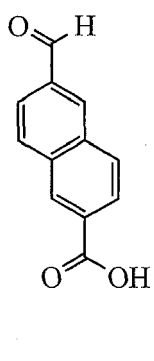
Aldehyde 1
