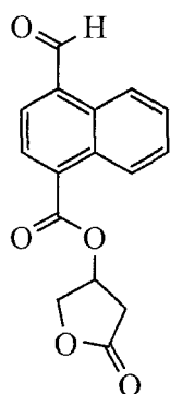
Aldehyde 2
