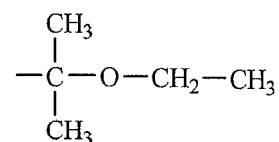
(A-2)-19
