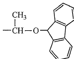
(A-2)-46
