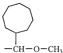
(A-2)-41
