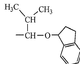
(A-2)-51
