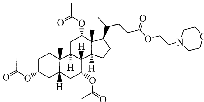
Quencher 2
