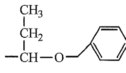
(A-2)-22
