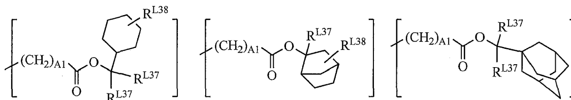
(A-1)-4
