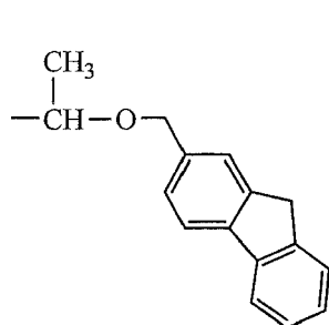
(A-2)-67
