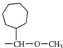
(A-2)-40
