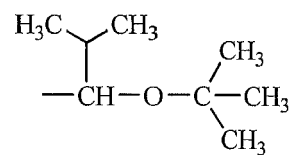
(A-2)-43
