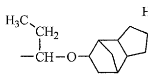
(A-2)-56
