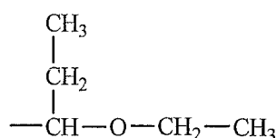
(A-2)-11
