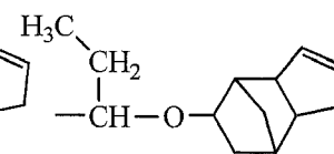
(A-2)-59
