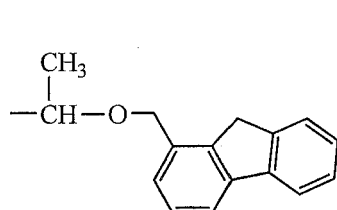
(A-2)-64
