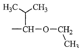
(A-2)-37
