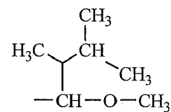
(A-2)-39
