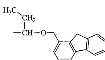
(A-2)-65
