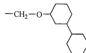
(A-2)-35
