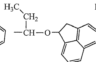
(A-2)-53
