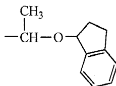
(A-2)-49
