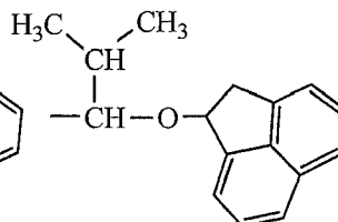
(A-2)-54
