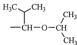
(A-2)-42
