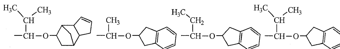
(A-2)-60
