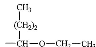
(A-2)-12
