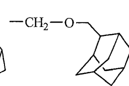
(A-2)-34
