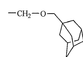
(A-2)-33
