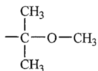
(A-2)-18
