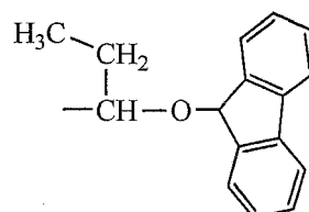
(A-2)-47
