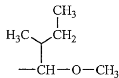
(A-2)-38
