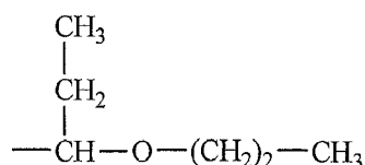
(A-2)-14
