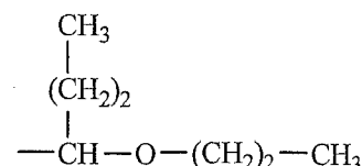
(A-2)-15
