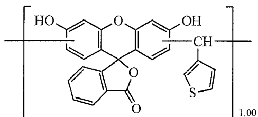
Novolak Resin 9 M_w = 2,100 M_w/M_n = 3.70
