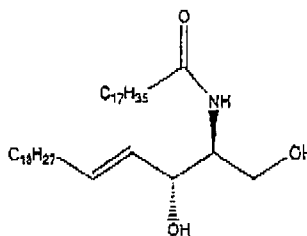
Ceramide
