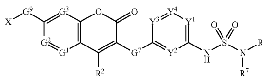
[Chemical Formula 32]
