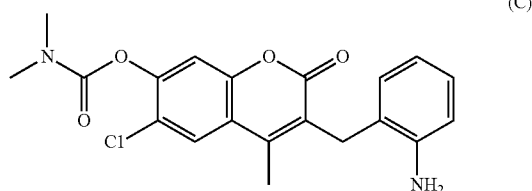
[Chemical Formula 14]
