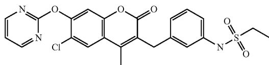
[Chemical Formula 26]
