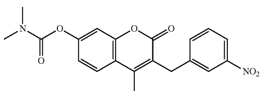
[Chemical Formula 74]
