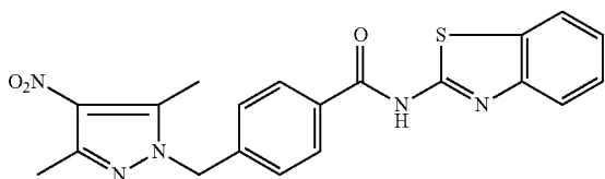
[Chemical Formula 27]
