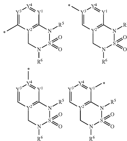
[Chemical Formula 29]
