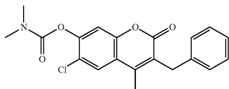
[Chemical Formula 27]
