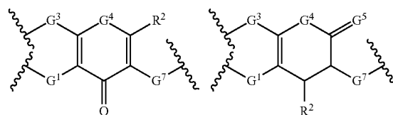
[Chemical Formula 18]
