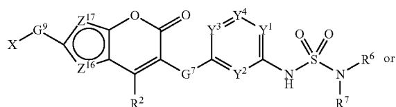
[Chemical Formula 45]
