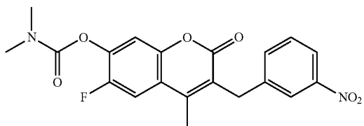
[Chemical Formula 75]
