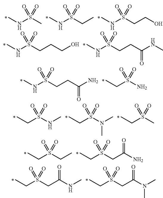
[Chemical Formula 28]
