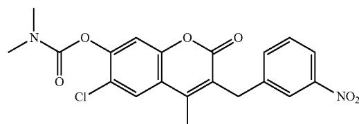
[Chemical Formula 76]
