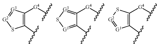
[Chemical Formula 16]
