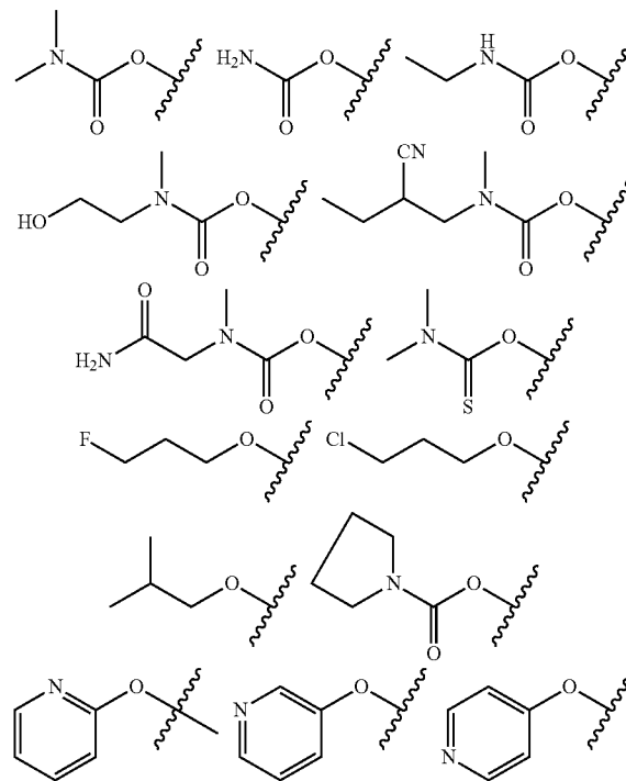
[Chemical Formula 4]
