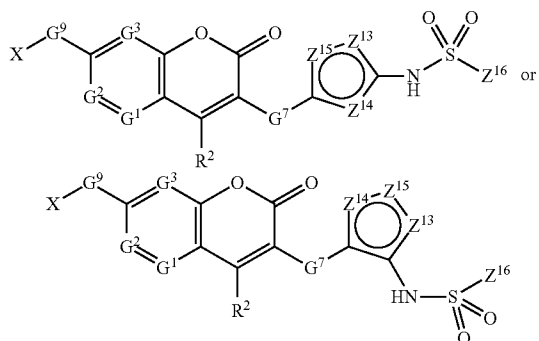
[Chemical Formula 44]
