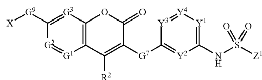
[Chemical Formula 42]
