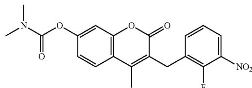
[Chemical Formula 77]
